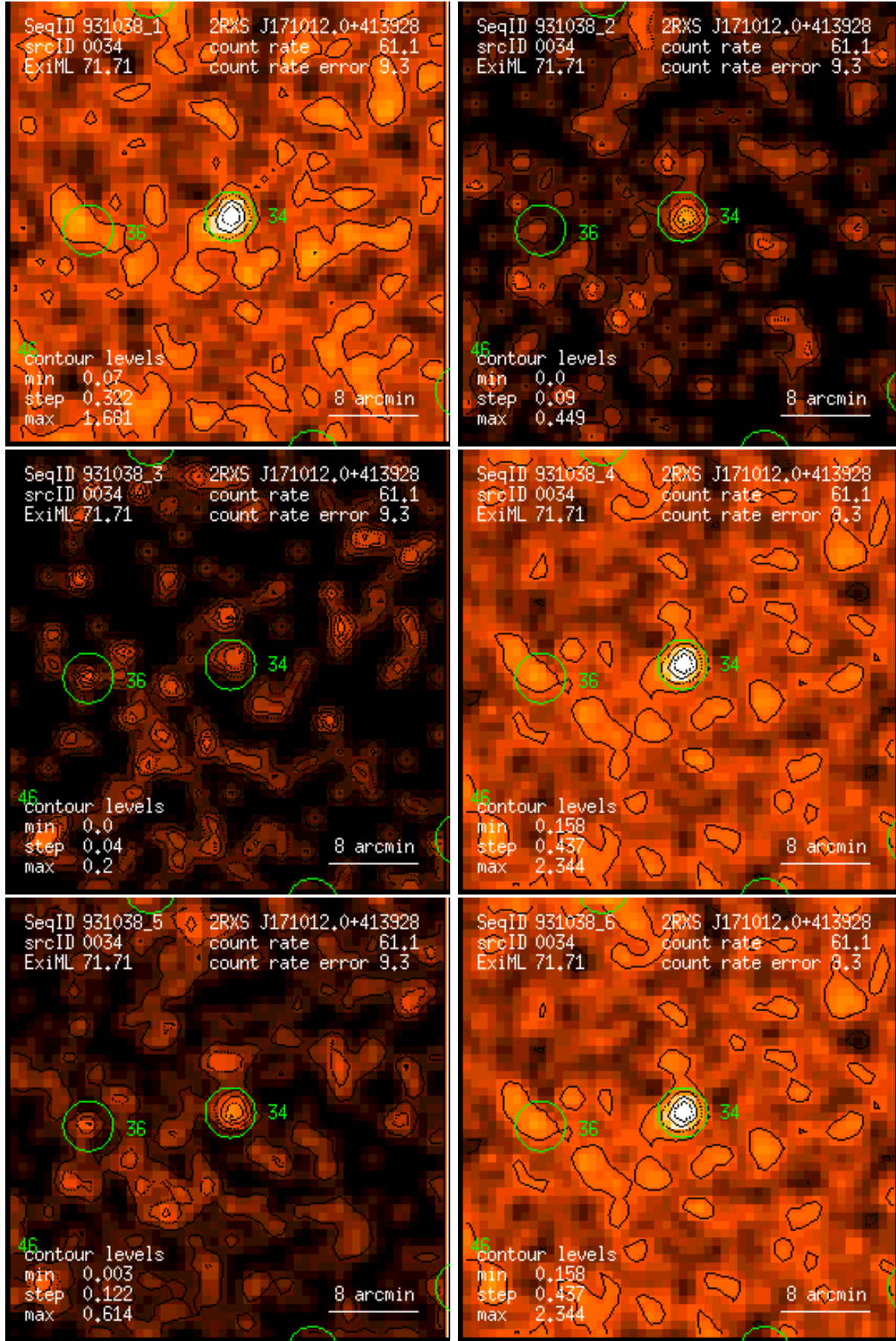
Figure 34: RASS 931038: detection 0034: band rate images, Gaussian filter: (1) PSPC channels 11 – 41, (2) 52 – 90, (3) 91 – 201, (4) 11 – 235, (5) 52 – 201, (6) 11 – 201. Broad band rates in counts/ks. Band rate contour levels in counts/ks/arcmin 2 .
