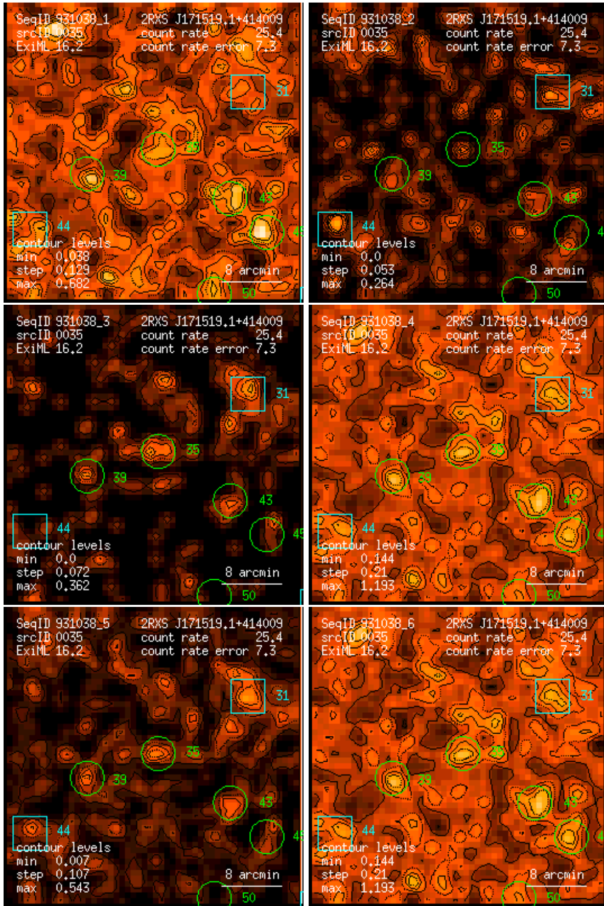
Figure 35: RASS 931038: detection 0035: band rate images, Gaussian filter: (1) PSPC channels 11 – 41, (2) 52 – 90, (3) 91 – 201, (4) 11 – 235, (5) 52 – 201, (6) 11 – 201. Broad band rates in counts/ks. Band rate contour levels in counts/ks/arcmin 2 .
