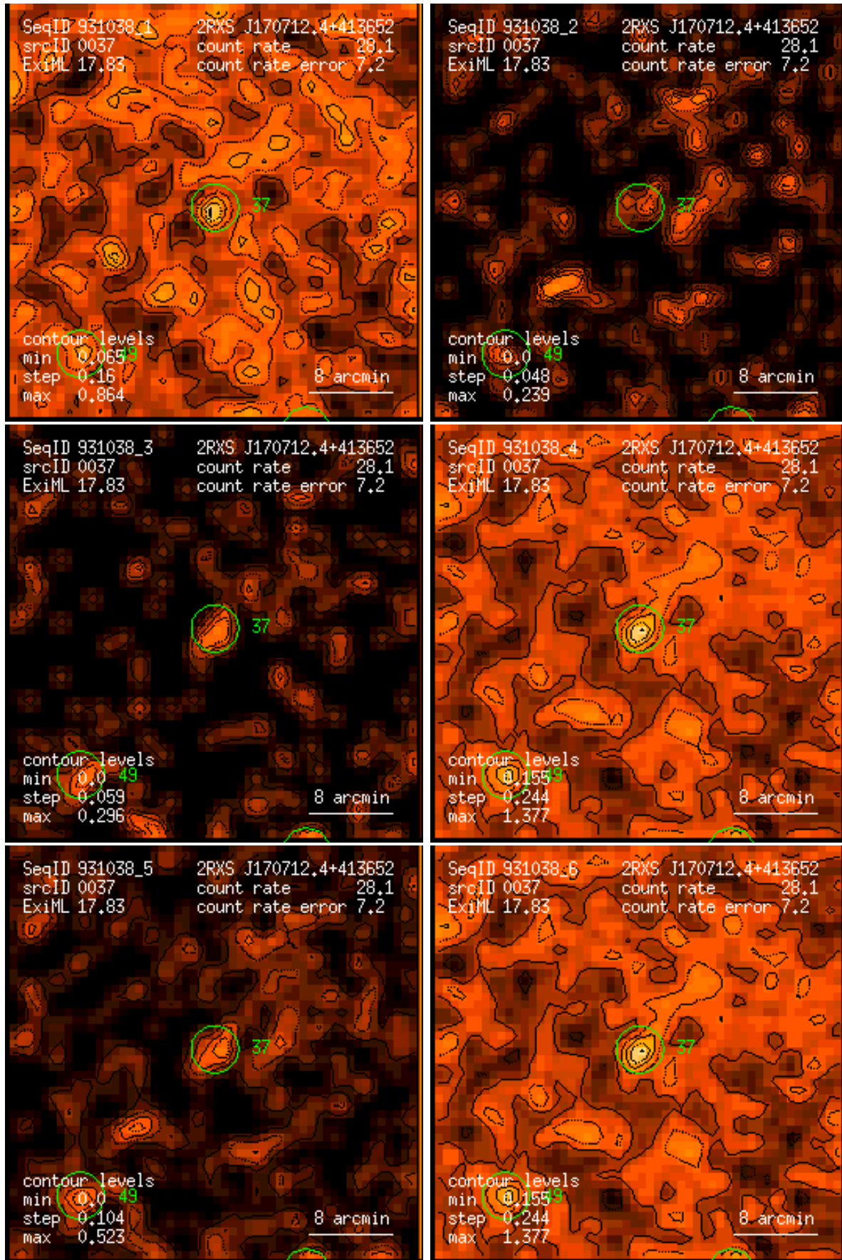
Figure 37: RASS 931038: detection 0037: band rate images, Gaussian filter: (1) PSPC channels 11 – 41, (2) 52 – 90, (3) 91 – 201, (4) 11 – 235, (5) 52 – 201, (6) 11 – 201. Broad band rates in counts/ks. Band rate contour levels in counts/ks/arcmin 2 .
