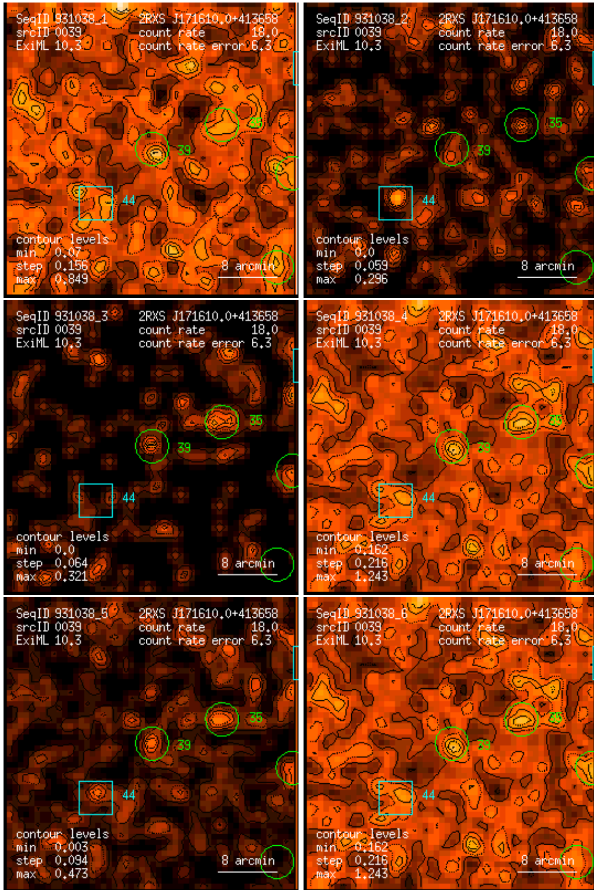
Figure 39: RASS 931038: detection 0039: band rate images, Gaussian filter: (1) PSPC channels 11 – 41, (2) 52 – 90, (3) 91 – 201, (4) 11 – 235, (5) 52 – 201, (6) 11 – 201. Broad band rates in counts/ks. Band rate contour levels in counts/ks/arcmin 2 .
