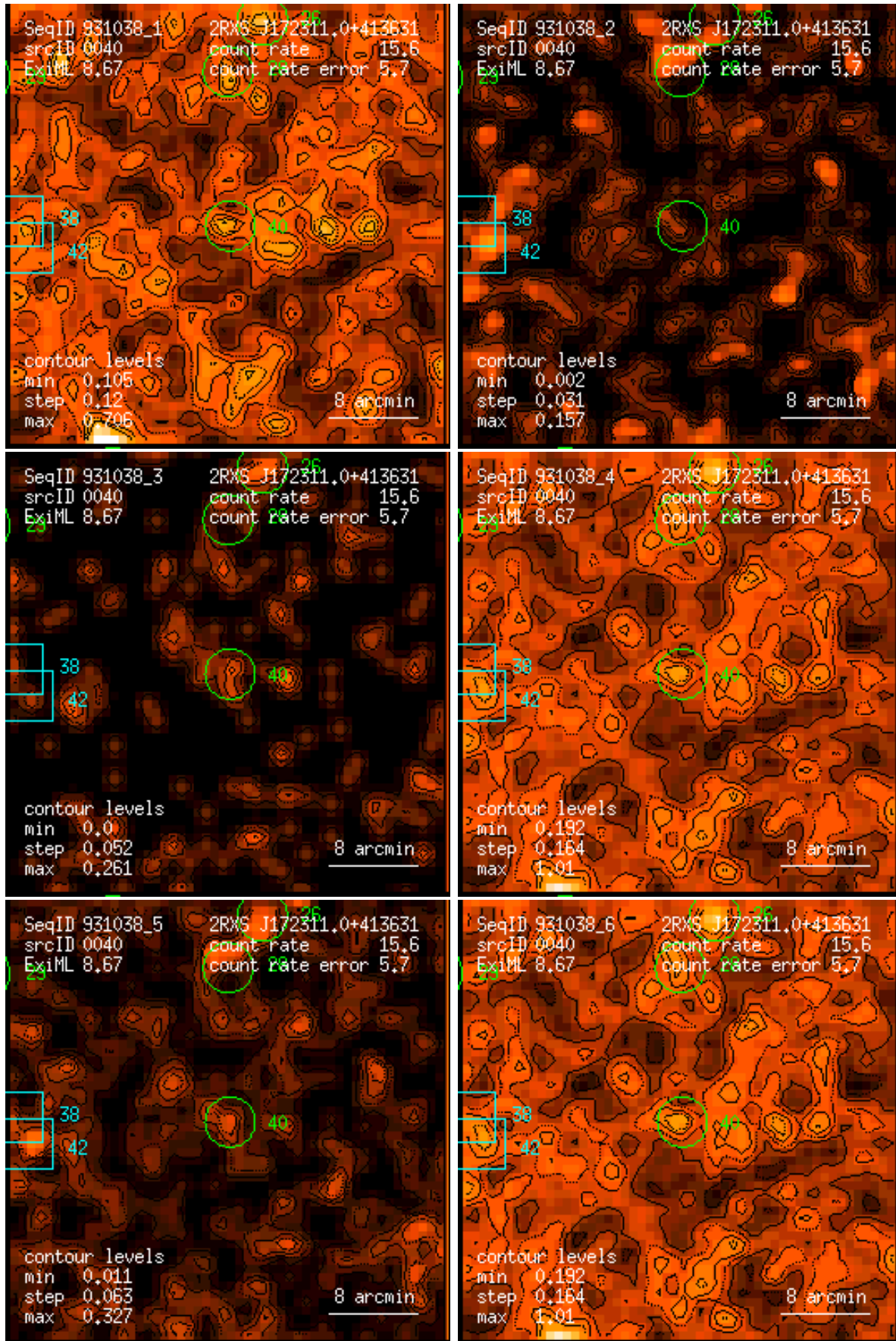
Figure 40: RASS 931038: detection 0040: band rate images, Gaussian filter: (1) PSPC channels 11 – 41, (2) 52 – 90, (3) 91 – 201, (4) 11 – 235, (5) 52 – 201, (6) 11 – 201. Broad band rates in counts/ks. Band rate contour levels in counts/ks/arcmin 2 .
