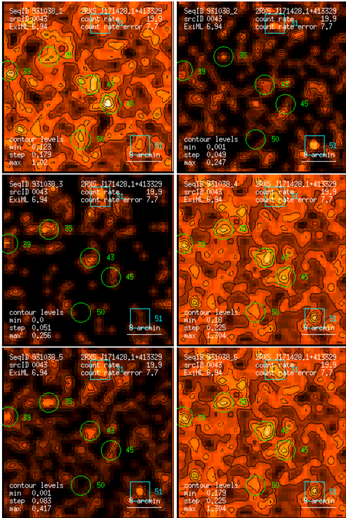
Figure 43: RASS 931038: detection 0043: band rate images, Gaussian filter: (1) PSPC channels 11 – 41, (2) 52 – 90, (3) 91 – 201, (4) 11 – 235, (5) 52 – 201, (6) 11 – 201. Broad band rates in counts/ks. Band rate contour levels in counts/ks/arcmin 2 .
