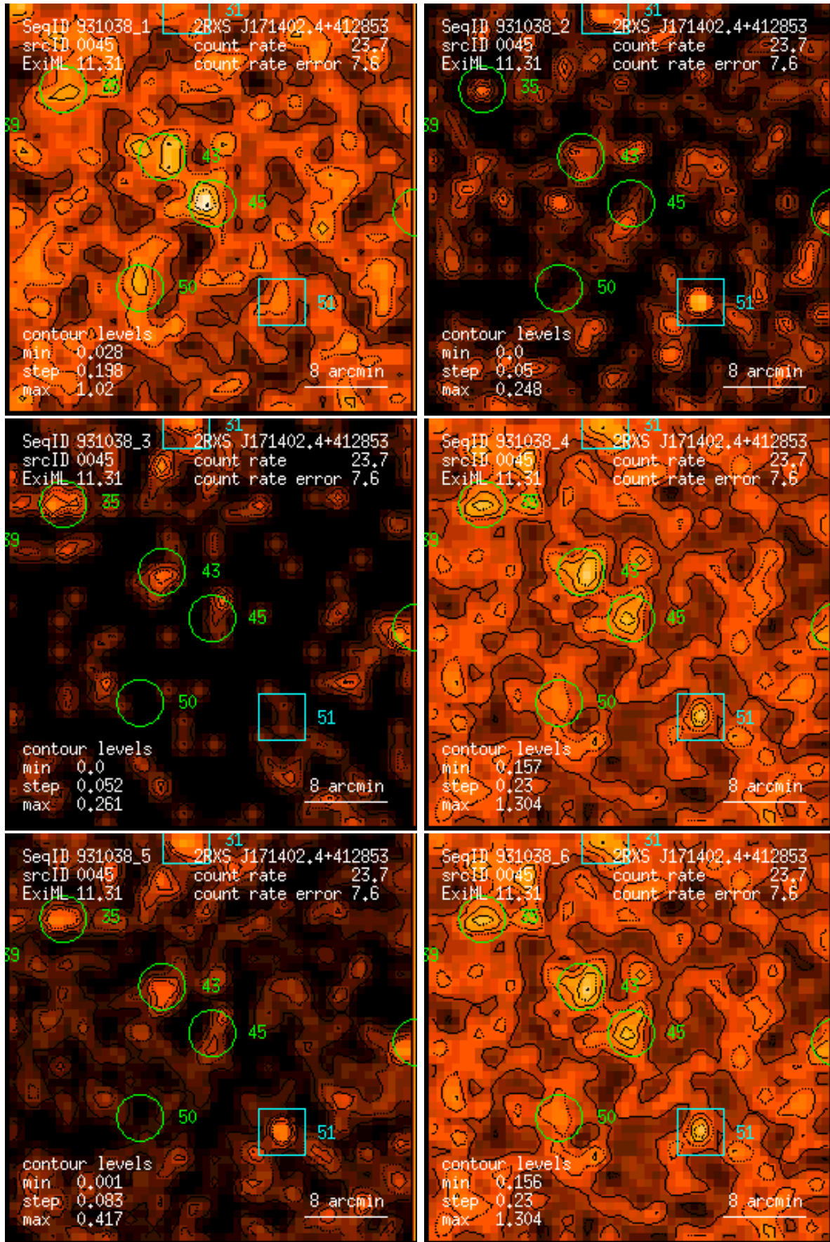
Figure 45: RASS 931038: detection 0045: band rate images, Gaussian filter: (1) PSPC channels 11 – 41, (2) 52 – 90, (3) 91 – 201, (4) 11 – 235, (5) 52 – 201, (6) 11 – 201. Broad band rates in counts/ks. Band rate contour levels in counts/ks/arcmin 2 .
