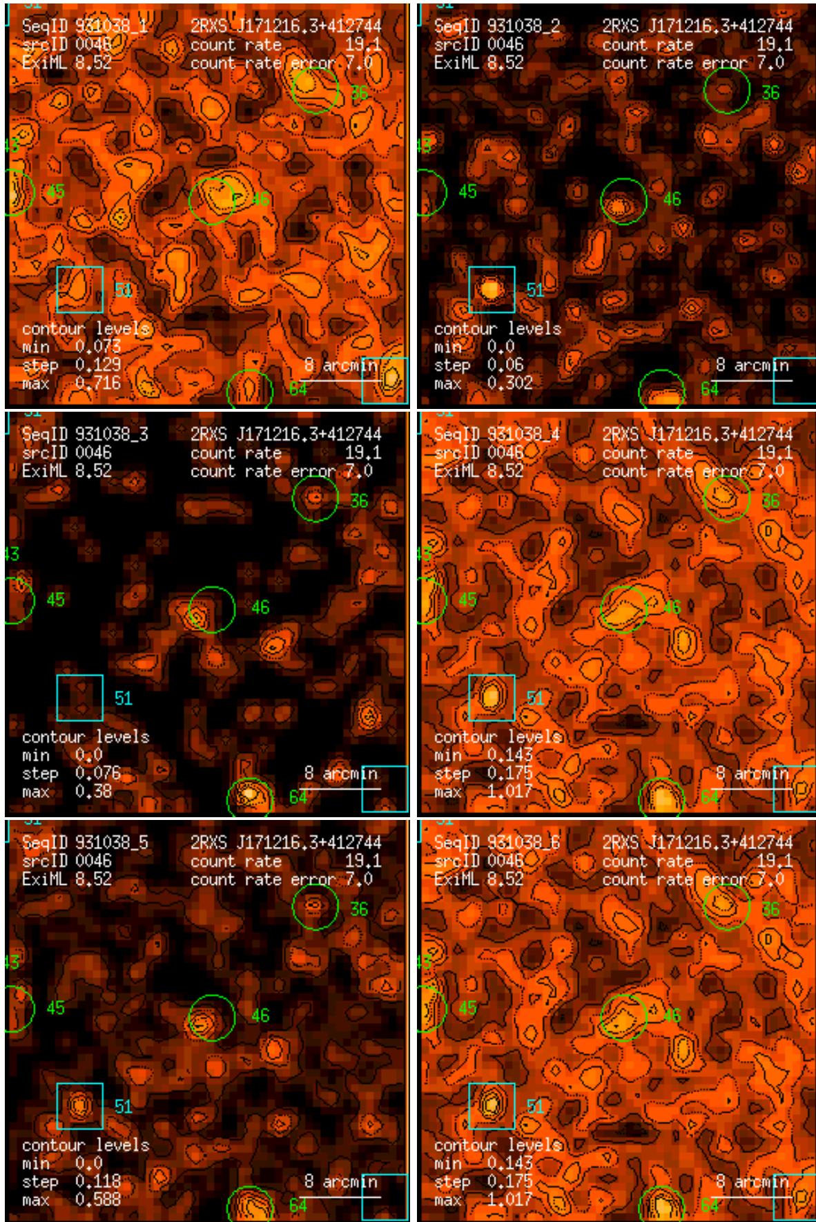
Figure 46: RASS 931038: detection 0046: band rate images, Gaussian filter: (1) PSPC channels 11 – 41, (2) 52 – 90, (3) 91 – 201, (4) 11 – 235, (5) 52 – 201, (6) 11 – 201. Broad band rates in counts/ks. Band rate contour levels in counts/ks/arcmin 2 .
