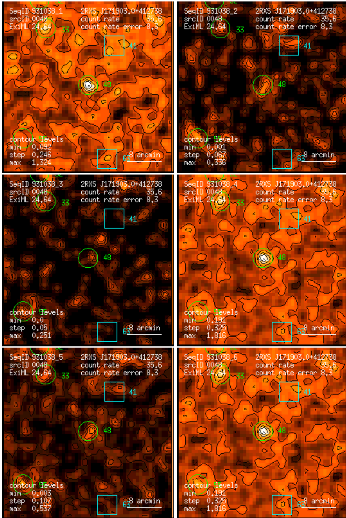
Figure 48: RASS 931038: detection 0048: band rate images, Gaussian filter: (1) PSPC channels 11 – 41, (2) 52 – 90, (3) 91 – 201, (4) 11 – 235, (5) 52 – 201, (6) 11 – 201. Broad band rates in counts/ks. Band rate contour levels in counts/ks/arcmin 2 .
