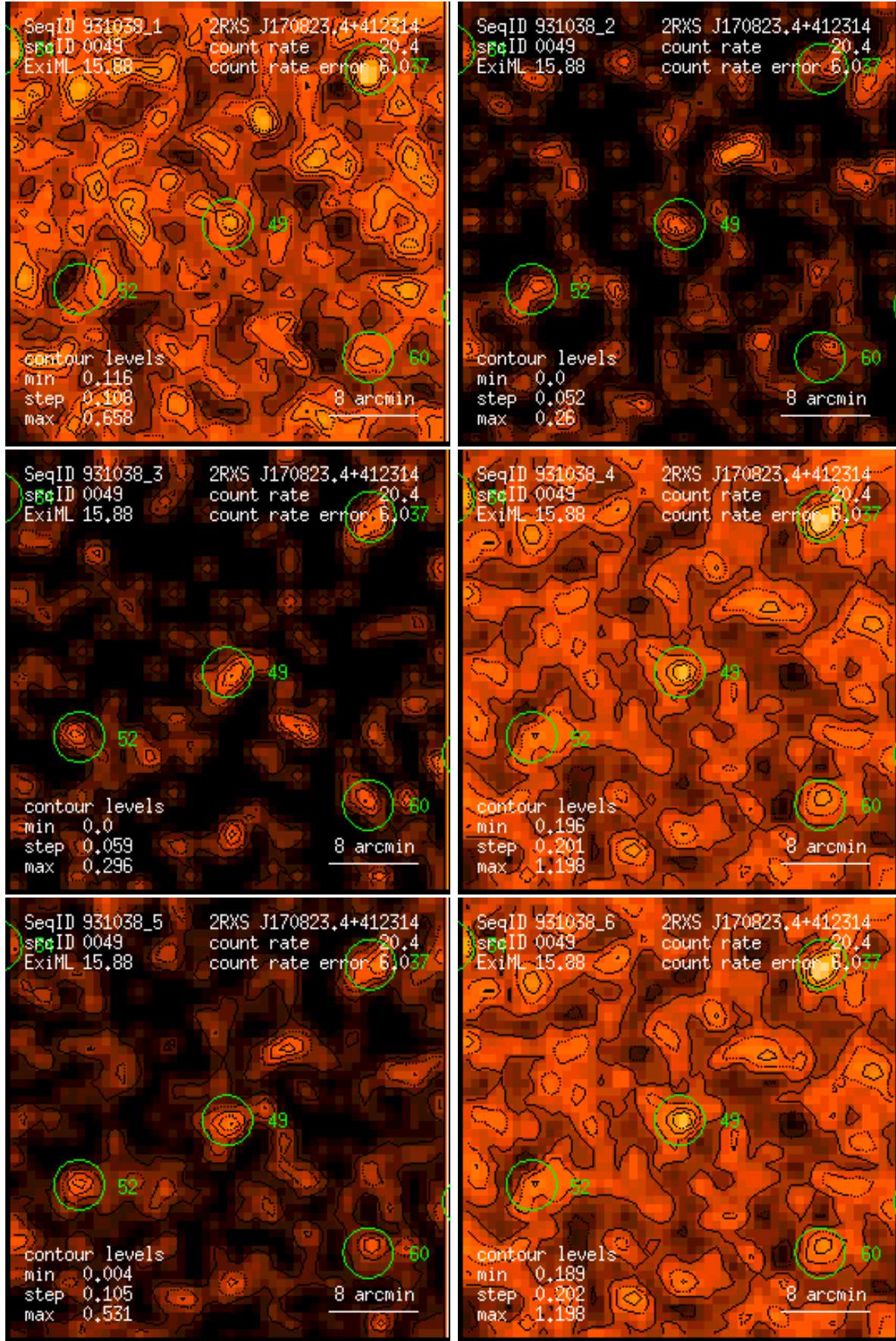
Figure 49: RASS 931038: detection 0049: band rate images, Gaussian filter: (1) PSPC channels 11 – 41, (2) 52 – 90, (3) 91 – 201, (4) 11 – 235, (5) 52 – 201, (6) 11 – 201. Broad band rates in counts/ks. Band rate contour levels in counts/ks/arcmin 2 .
