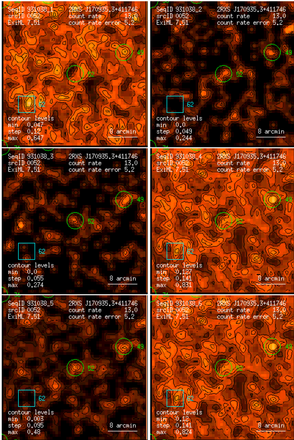
Figure 52: RASS 931038: detection 0052: band rate images, Gaussian filter: (1) PSPC channels 11 – 41, (2) 52 – 90, (3) 91 – 201, (4) 11 – 235, (5) 52 – 201, (6) 11 – 201. Broad band rates in counts/ks. Band rate contour levels in counts/ks/arcmin 2 .
