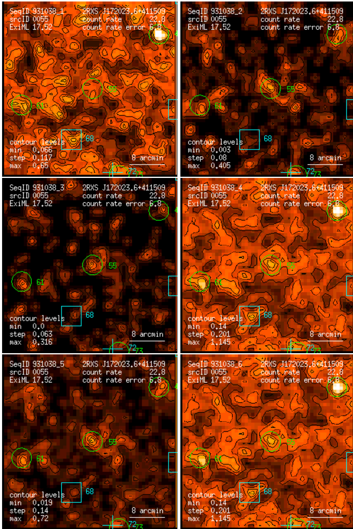
Figure 55: RASS 931038: detection 0055: band rate images, Gaussian filter: (1) PSPC channels 11 – 41, (2) 52 – 90, (3) 91 – 201, (4) 11 – 235, (5) 52 – 201, (6) 11 – 201. Broad band rates in counts/ks. Band rate contour levels in counts/ks/arcmin 2 .
