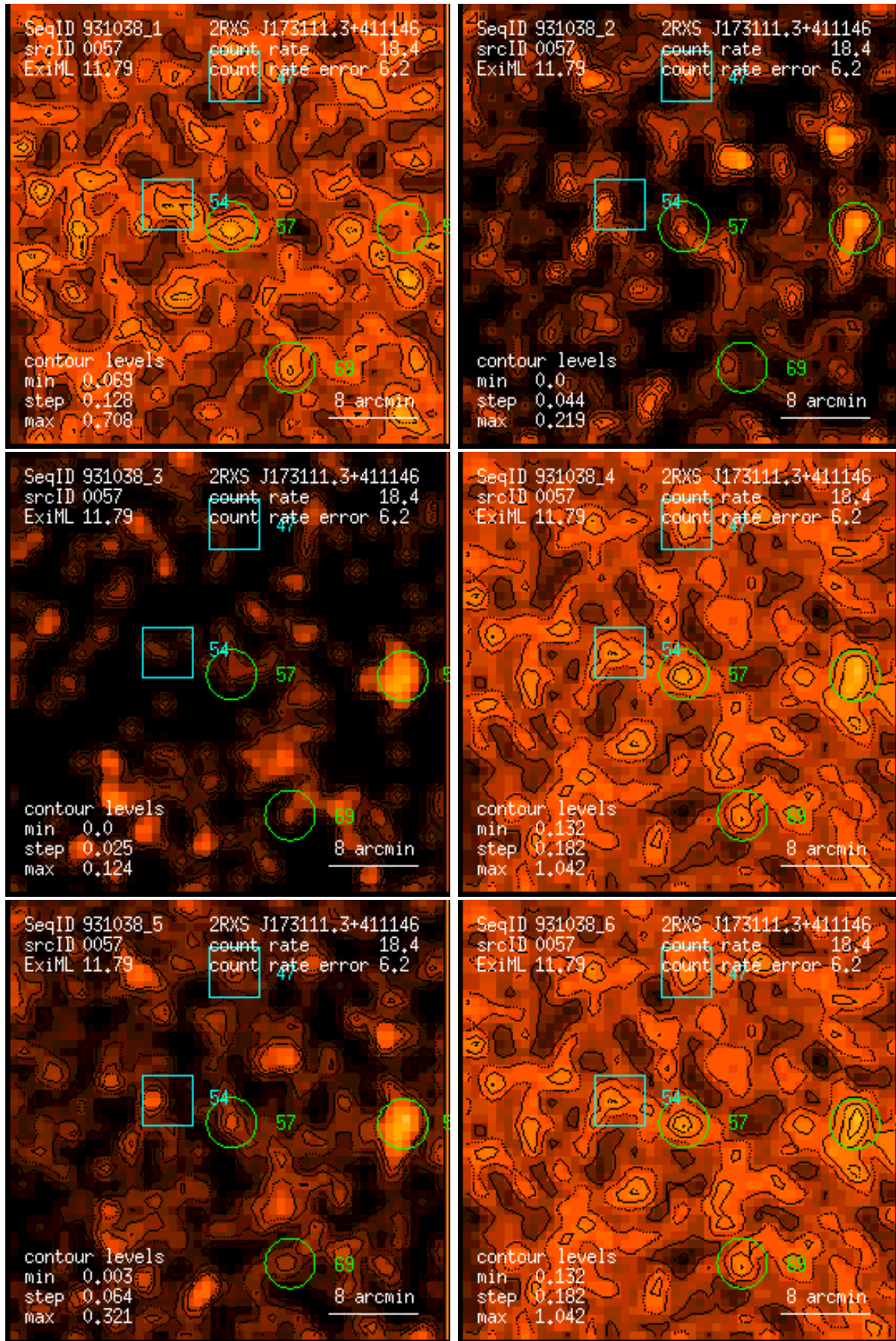
Figure 57: RASS 931038: detection 0057: band rate images, Gaussian filter: (1) PSPC channels 11 – 41, (2) 52 – 90, (3) 91 – 201, (4) 11 – 235, (5) 52 – 201, (6) 11 – 201. Broad band rates in counts/ks. Band rate contour levels in counts/ks/arcmin 2 .
