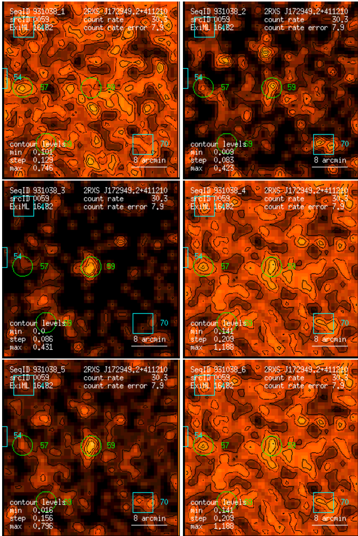
Figure 59: RASS 931038: detection 0059: band rate images, Gaussian filter: (1) PSPC channels 11 – 41, (2) 52 – 90, (3) 91 – 201, (4) 11 – 235, (5) 52 – 201, (6) 11 – 201. Broad band rates in counts/ks. Band rate contour levels in counts/ks/arcmin 2 .
