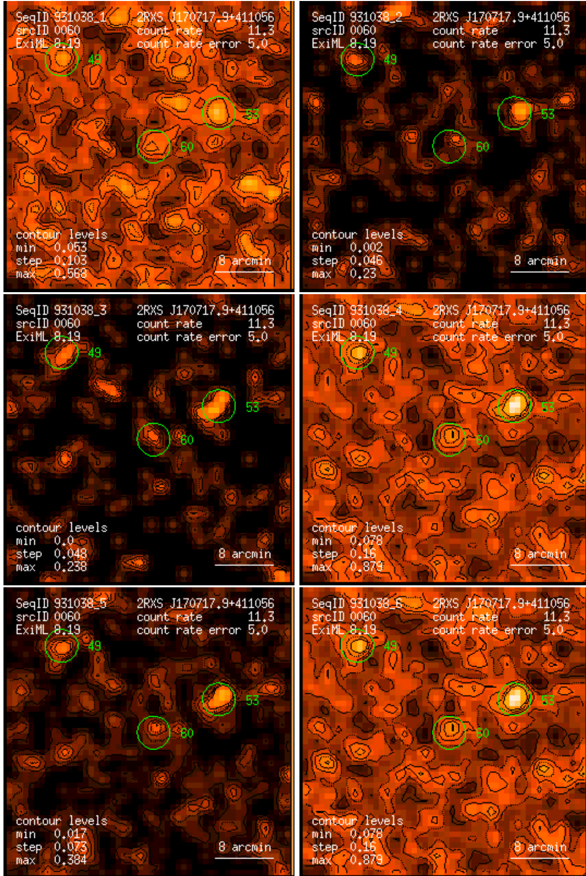
Figure 60: RASS 931038: detection 0060: band rate images, Gaussian filter: (1) PSPC channels 11 – 41, (2) 52 – 90, (3) 91 – 201, (4) 11 – 235, (5) 52 – 201, (6) 11 – 201. Broad band rates in counts/ks. Band rate contour levels in counts/ks/arcmin 2 .
