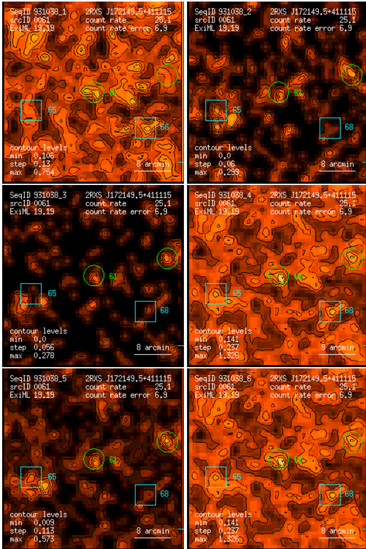
Figure 61: RASS 931038: detection 0061: band rate images, Gaussian filter: (1) PSPC channels 11 – 41, (2) 52 – 90, (3) 91 – 201, (4) 11 – 235, (5) 52 – 201, (6) 11 – 201. Broad band rates in counts/ks. Band rate contour levels in counts/ks/arcmin 2 .
