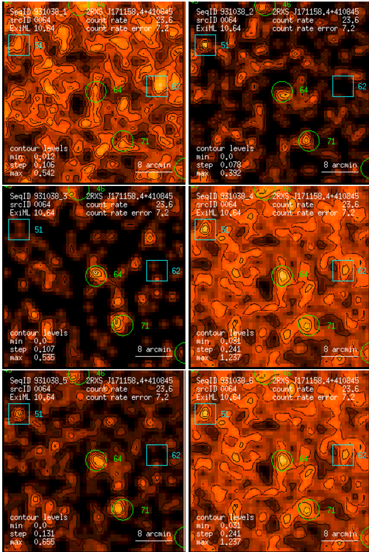
Figure 64: RASS 931038: detection 0064: band rate images, Gaussian filter: (1) PSPC channels 11 – 41, (2) 52 – 90, (3) 91 – 201, (4) 11 – 235, (5) 52 – 201, (6) 11 – 201. Broad band rates in counts/ks. Band rate contour levels in counts/ks/arcmin 2 .
