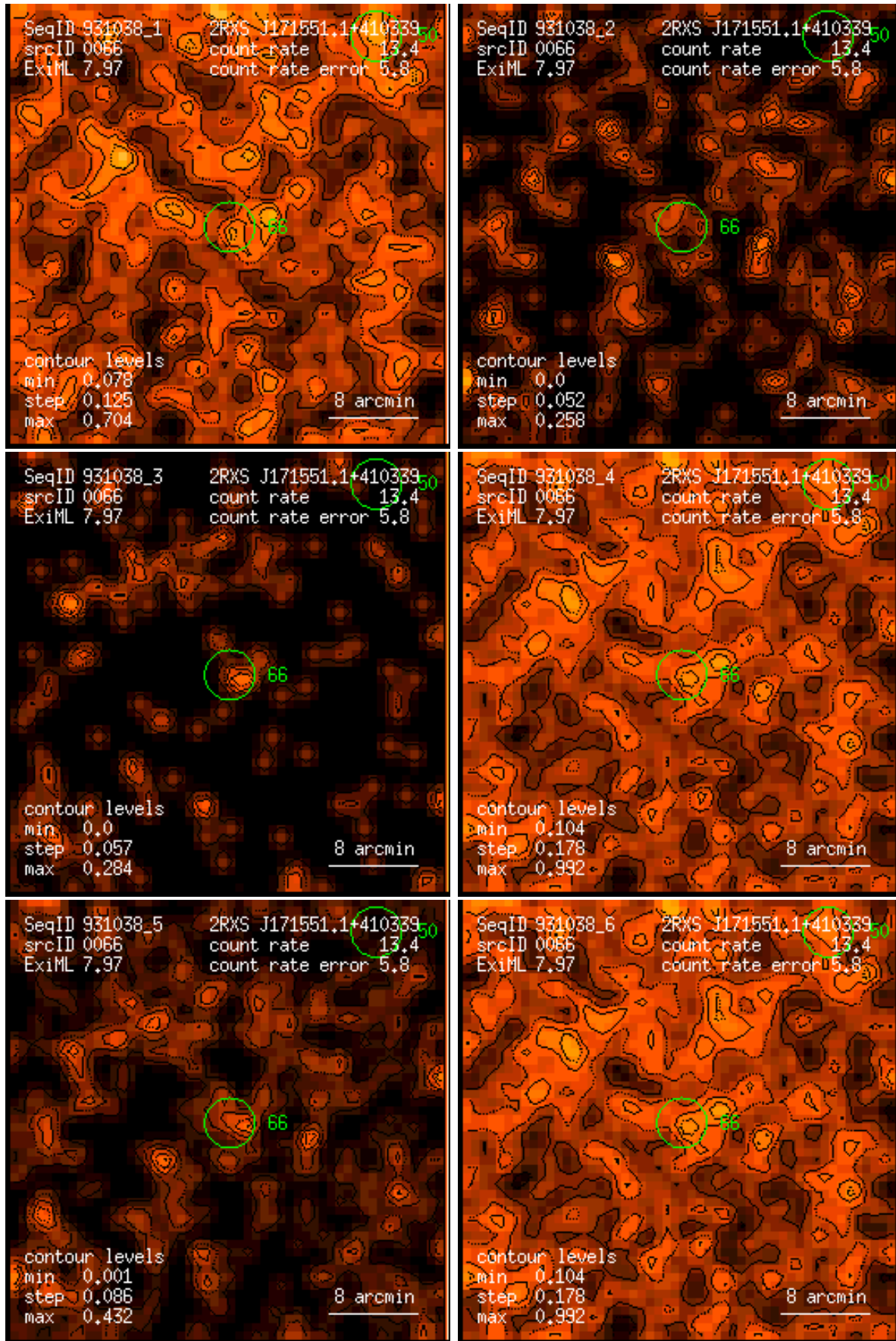
Figure 66: RASS 931038: detection 0066: band rate images, Gaussian filter: (1) PSPC channels 11 – 41, (2) 52 – 90, (3) 91 – 201, (4) 11 – 235, (5) 52 – 201, (6) 11 – 201. Broad band rates in counts/ks. Band rate contour levels in counts/ks/arcmin 2 .
