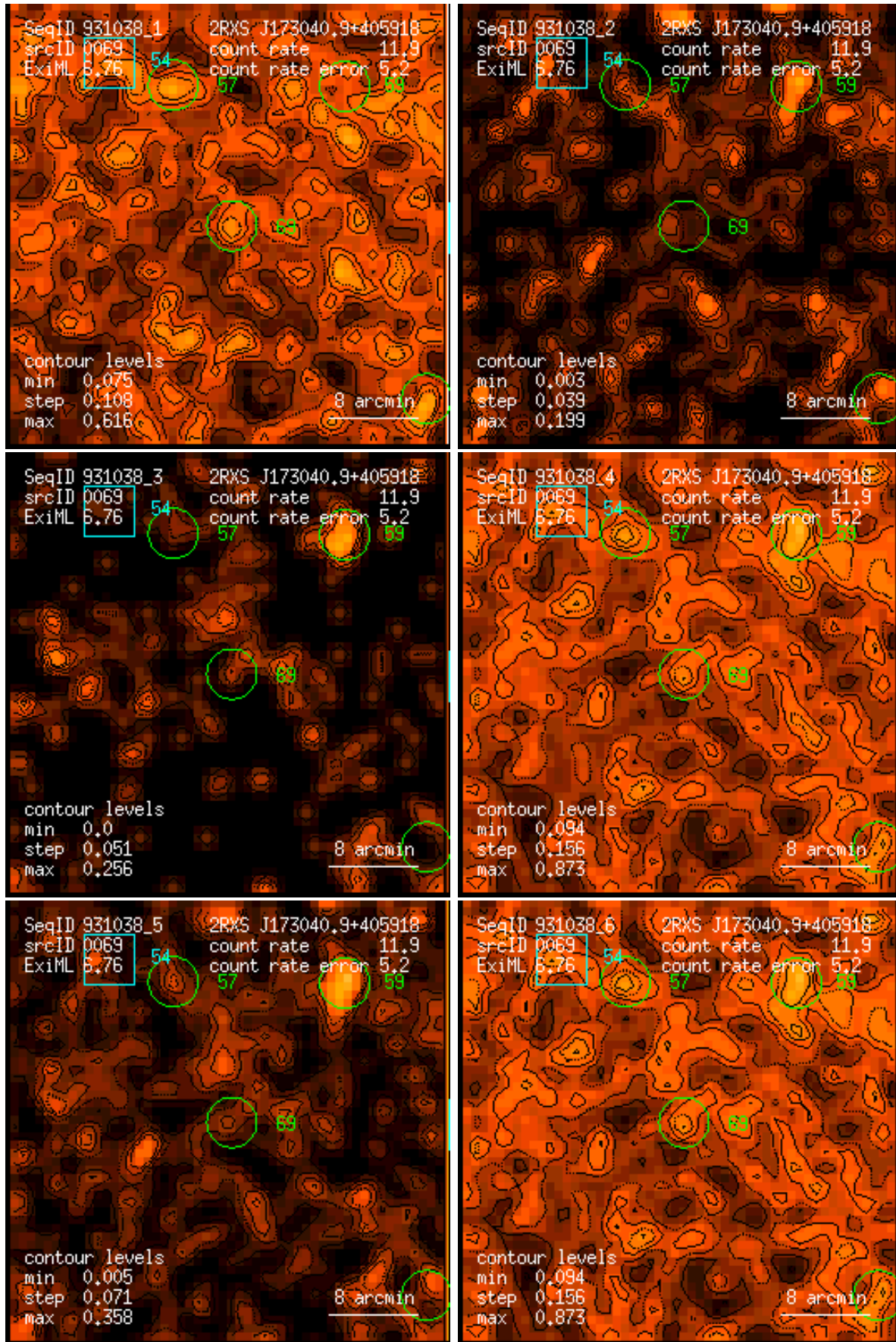
Figure 69: RASS 931038: detection 0069: band rate images, Gaussian filter: (1) PSPC channels 11 – 41, (2) 52 – 90, (3) 91 – 201, (4) 11 – 235, (5) 52 – 201, (6) 11 – 201. Broad band rates in counts/ks. Band rate contour levels in counts/ks/arcmin 2 .
