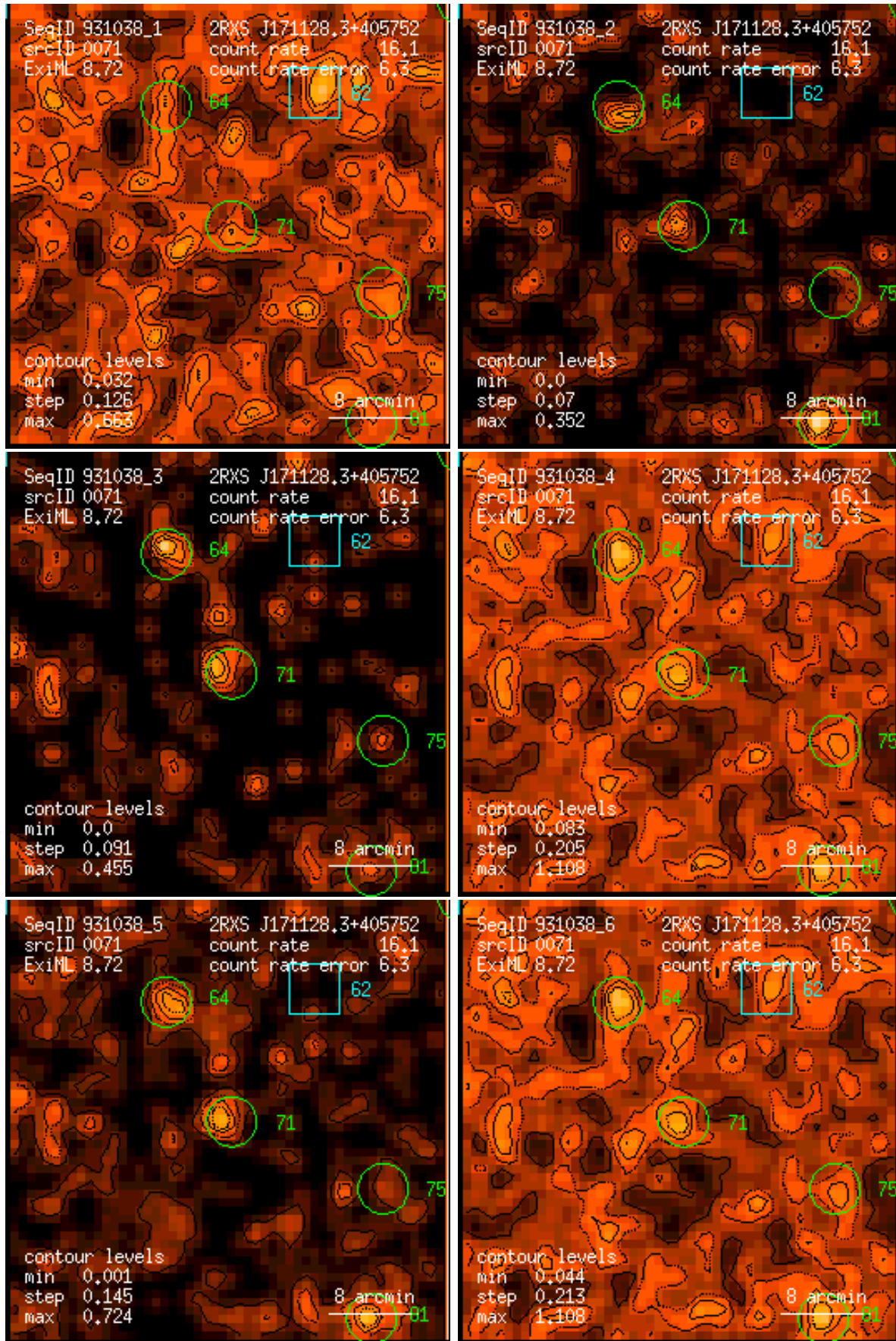
Figure 71: RASS 931038: detection 0071: band rate images, Gaussian filter: (1) PSPC channels 11 – 41, (2) 52 – 90, (3) 91 – 201, (4) 11 – 235, (5) 52 – 201, (6) 11 – 201. Broad band rates in counts/ks. Band rate contour levels in counts/ks/arcmin 2 .
