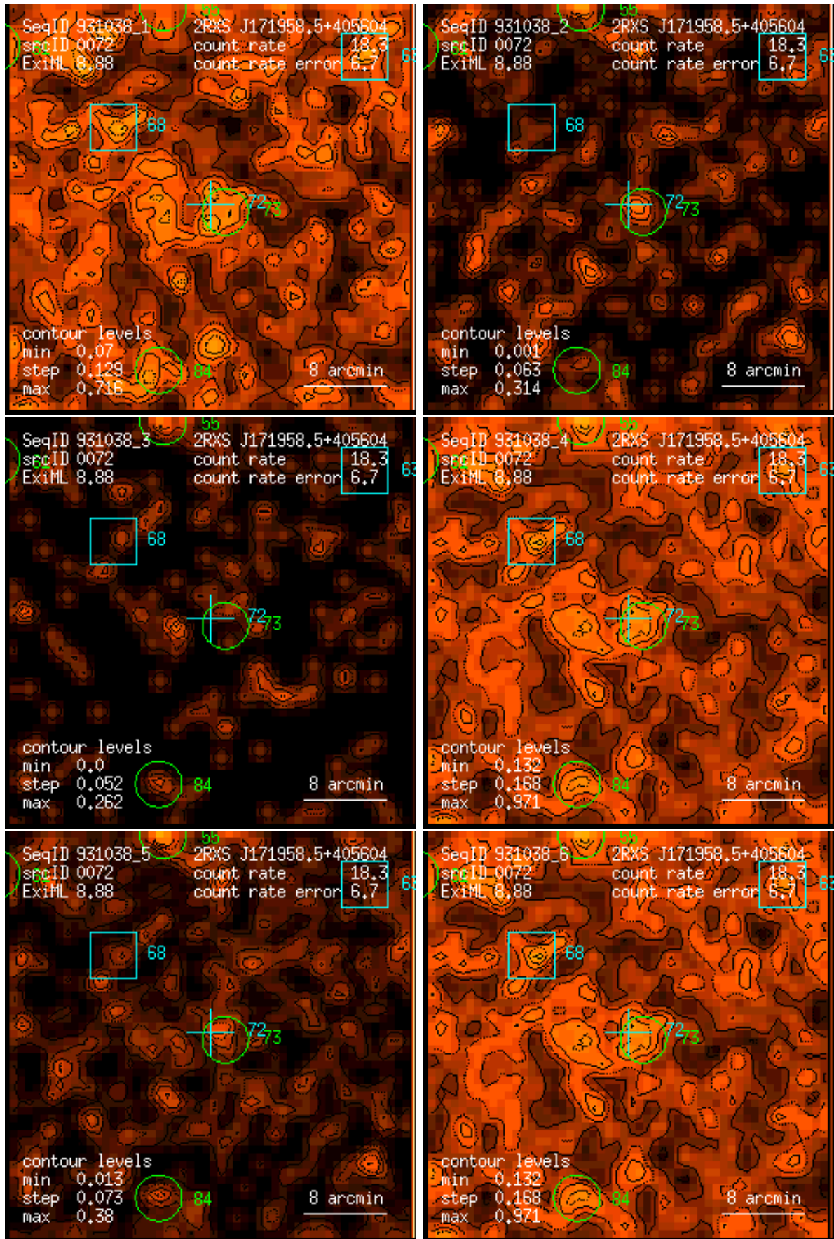
Figure 72: RASS 931038: detection 0072: band rate images, Gaussian filter: (1) PSPC channels 11 – 41, (2) 52 – 90, (3) 91 – 201, (4) 11 – 235, (5) 52 – 201, (6) 11 – 201. Broad band rates in counts/ks. Band rate contour levels in counts/ks/arcmin 2 .
