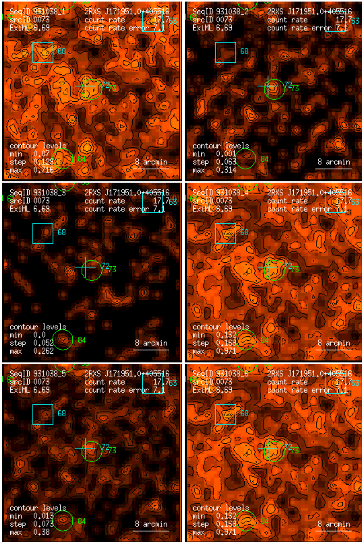
Figure 73: RASS 931038: detection 0073: band rate images, Gaussian filter: (1) PSPC channels 11 – 41, (2) 52 – 90, (3) 91 – 201, (4) 11 – 235, (5) 52 – 201, (6) 11 – 201. Broad band rates in counts/ks. Band rate contour levels in counts/ks/arcmin 2 .
