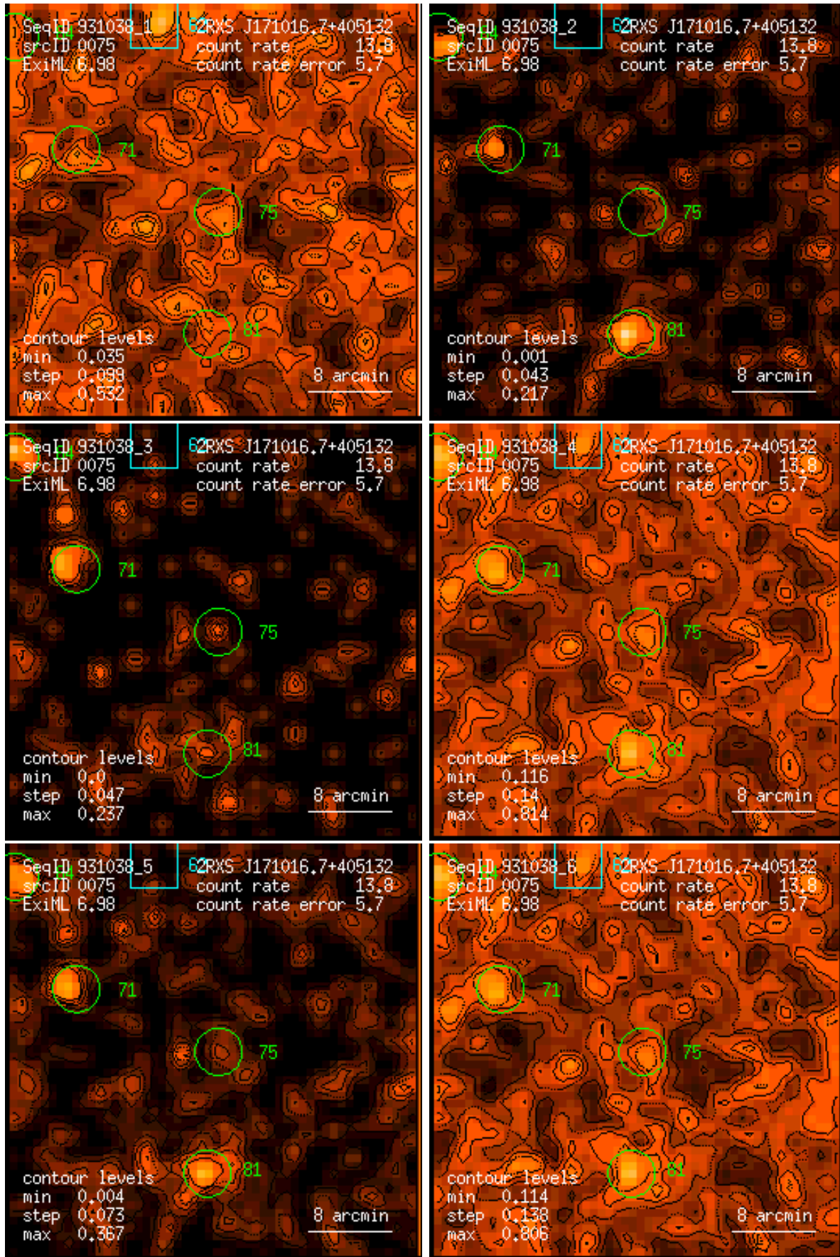
Figure 75: RASS 931038: detection 0075: band rate images, Gaussian filter: (1) PSPC channels 11 – 41, (2) 52 – 90, (3) 91 – 201, (4) 11 – 235, (5) 52 – 201, (6) 11 – 201. Broad band rates in counts/ks. Band rate contour levels in counts/ks/arcmin 2 .
