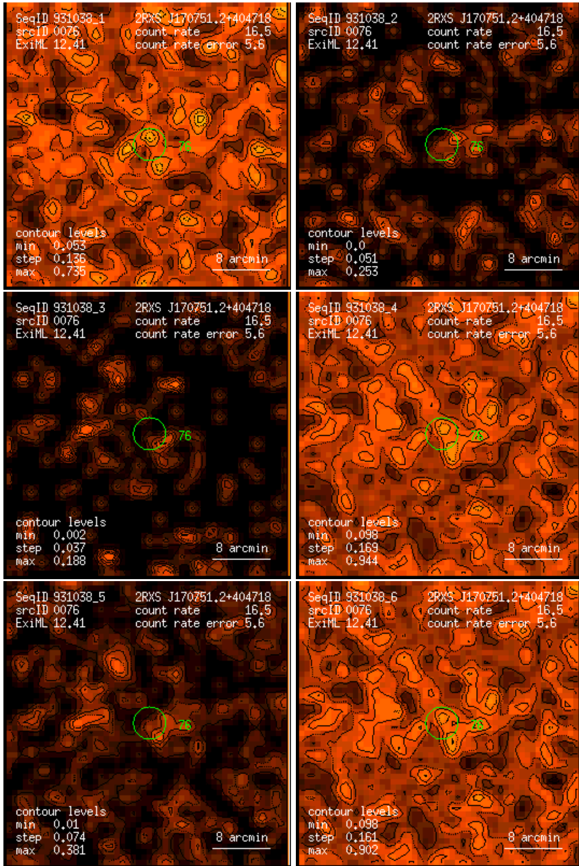
Figure 76: RASS 931038: detection 0076: band rate images, Gaussian filter: (1) PSPC channels 11 – 41, (2) 52 – 90, (3) 91 – 201, (4) 11 – 235, (5) 52 – 201, (6) 11 – 201. Broad band rates in counts/ks. Band rate contour levels in counts/ks/arcmin 2 .
