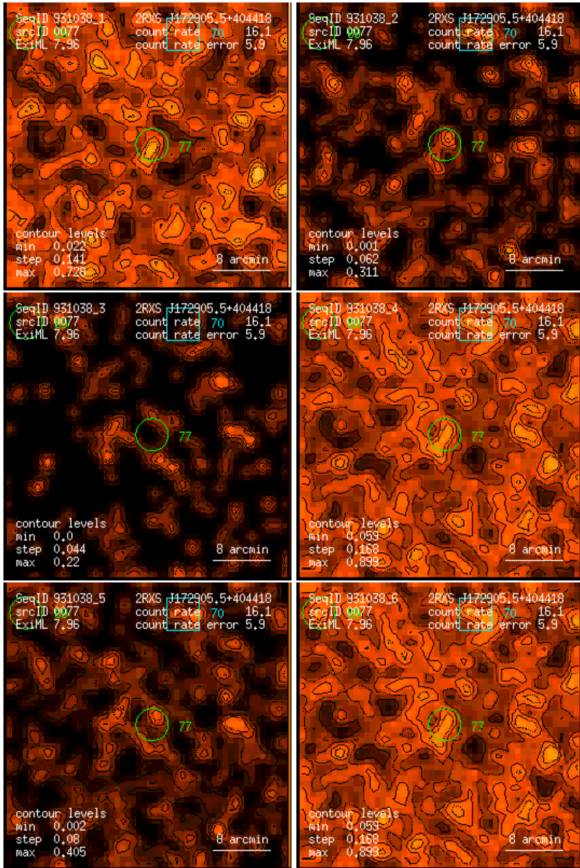
Figure 77: RASS 931038: detection 0077: band rate images, Gaussian filter: (1) PSPC channels 11 – 41, (2) 52 – 90, (3) 91 – 201, (4) 11 – 235, (5) 52 – 201, (6) 11 – 201. Broad band rates in counts/ks. Band rate contour levels in counts/ks/arcmin 2 .
