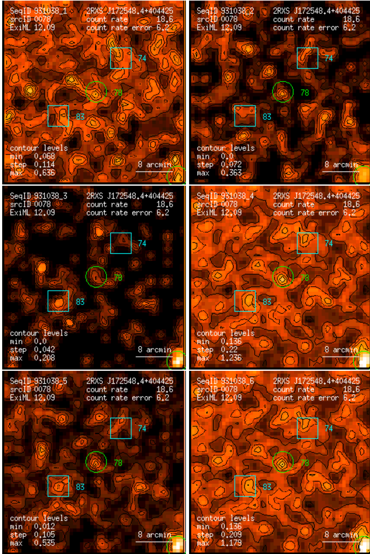
Figure 78: RASS 931038: detection 0078: band rate images, Gaussian filter: (1) PSPC channels 11 – 41, (2) 52 – 90, (3) 91 – 201, (4) 11 – 235, (5) 52 – 201, (6) 11 – 201. Broad band rates in counts/ks. Band rate contour levels in counts/ks/arcmin 2 .
