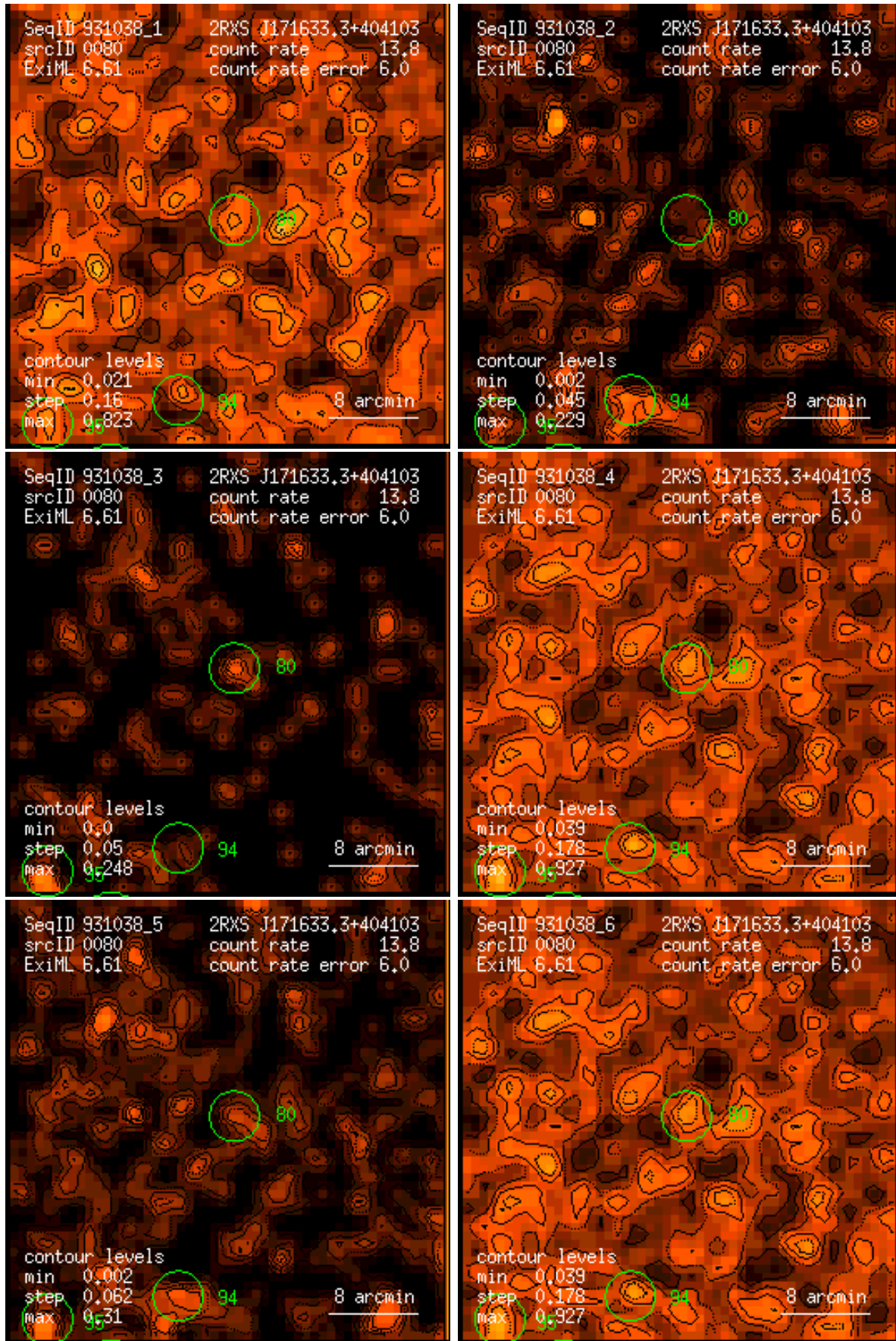
Figure 80: RASS 931038: detection 0080: band rate images, Gaussian filter: (1) PSPC channels 11 – 41, (2) 52 – 90, (3) 91 – 201, (4) 11 – 235, (5) 52 – 201, (6) 11 – 201. Broad band rates in counts/ks. Band rate contour levels in counts/ks/arcmin 2 .
