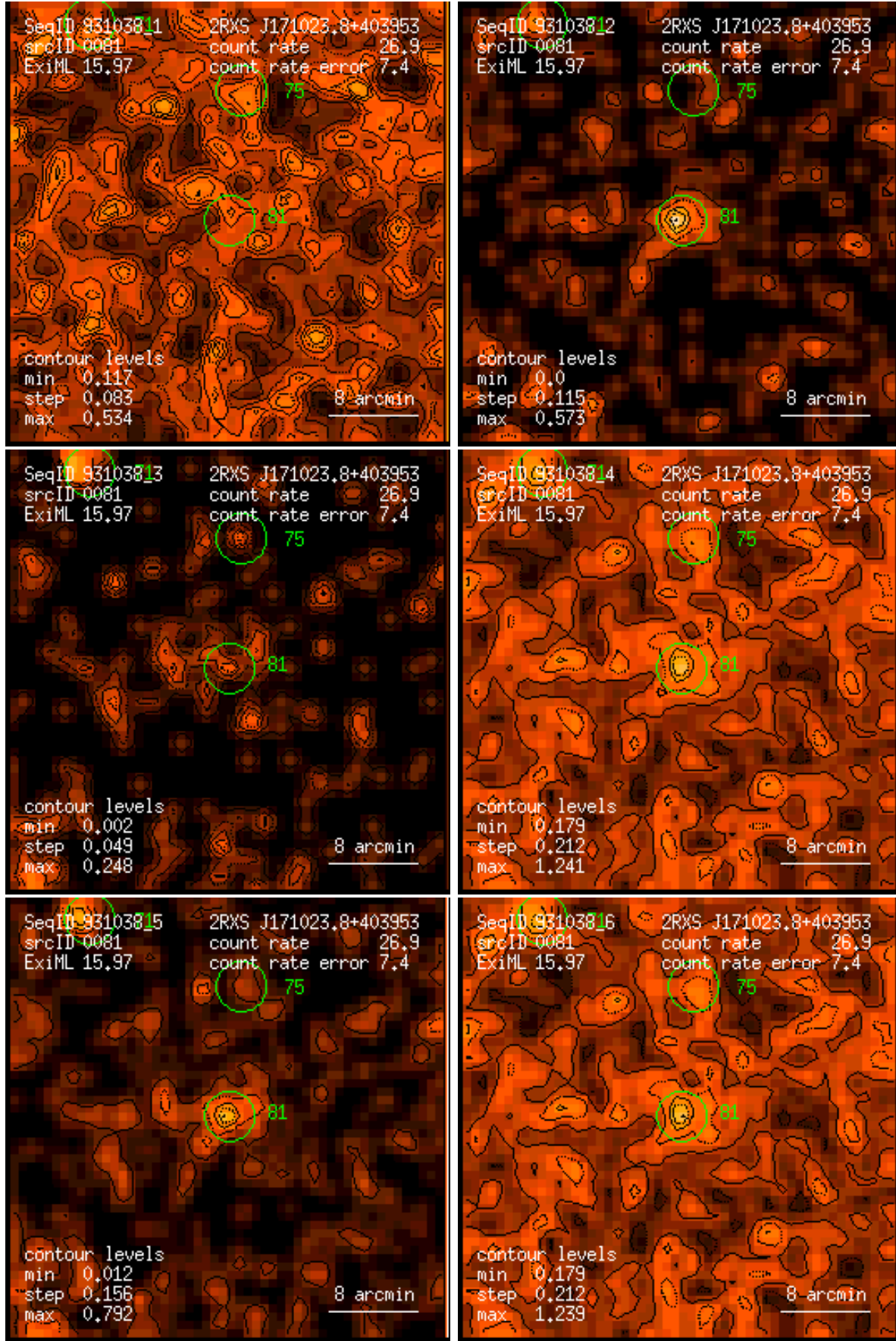
Figure 81: RASS 931038: detection 0081: band rate images, Gaussian filter: (1) PSPC channels 11 – 41, (2) 52 – 90, (3) 91 – 201, (4) 11 – 235, (5) 52 – 201, (6) 11 – 201. Broad band rates in counts/ks. Band rate contour levels in counts/ks/arcmin 2 .
