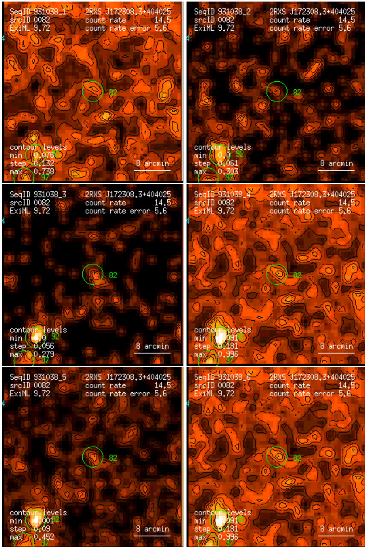
Figure 82: RASS 931038: detection 0082: band rate images, Gaussian filter: (1) PSPC channels 11 – 41, (2) 52 – 90, (3) 91 – 201, (4) 11 – 235, (5) 52 – 201, (6) 11 – 201. Broad band rates in counts/ks. Band rate contour levels in counts/ks/arcmin 2 .
