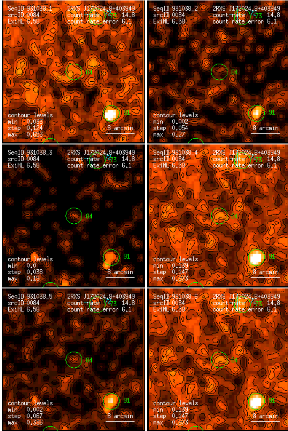
Figure 84: RASS 931038: detection 0084: band rate images, Gaussian filter: (1) PSPC channels 11 – 41, (2) 52 – 90, (3) 91 – 201, (4) 11 – 235, (5) 52 – 201, (6) 11 – 201. Broad band rates in counts/ks. Band rate contour levels in counts/ks/arcmin 2 .
