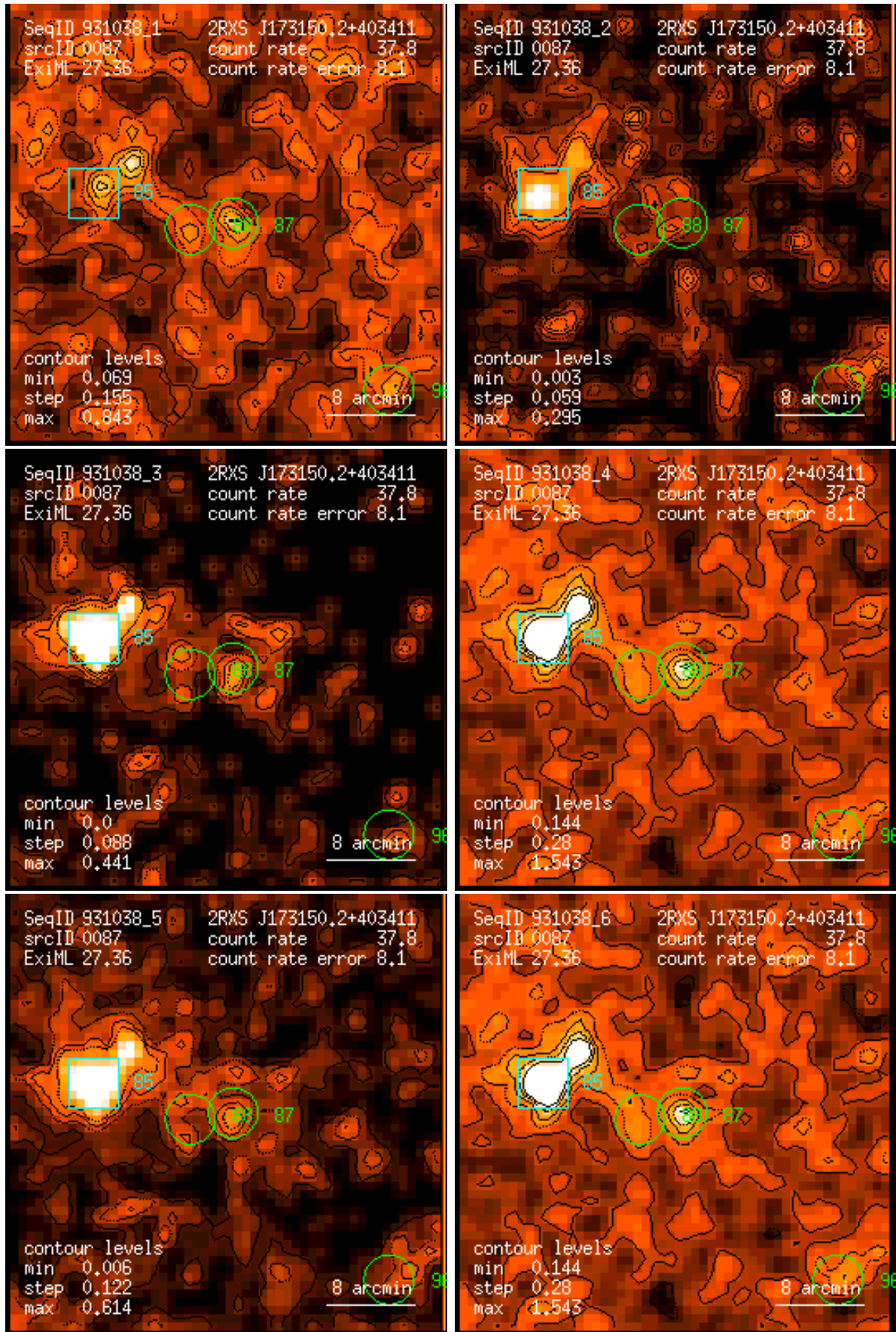
Figure 87: RASS 931038: detection 0087: band rate images, Gaussian filter: (1) PSPC channels 11 – 41, (2) 52 – 90, (3) 91 – 201, (4) 11 – 235, (5) 52 – 201, (6) 11 – 201. Broad band rates in counts/ks. Band rate contour levels in counts/ks/arcmin 2 .
