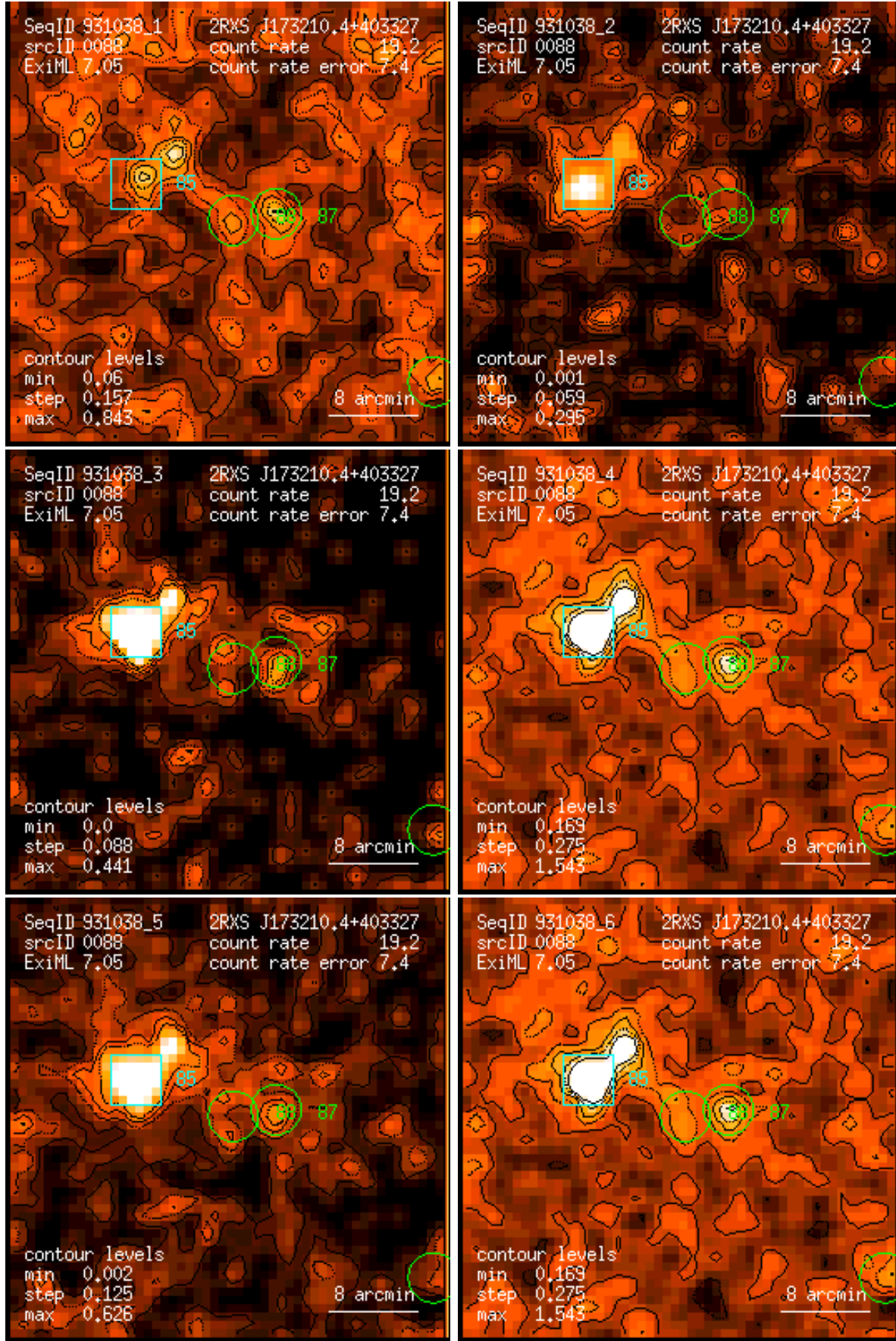
Figure 88: RASS 931038: detection 0088: band rate images, Gaussian filter: (1) PSPC channels 11 – 41, (2) 52 – 90, (3) 91 – 201, (4) 11 – 235, (5) 52 – 201, (6) 11 – 201. Broad band rates in counts/ks. Band rate contour levels in counts/ks/arcmin 2 .
