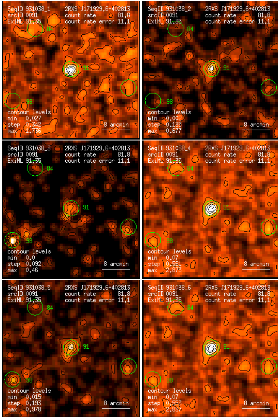
Figure 91: RASS 931038: detection 0091: band rate images, Gaussian filter: (1) PSPC channels 11 – 41, (2) 52 – 90, (3) 91 – 201, (4) 11 – 235, (5) 52 – 201, (6) 11 – 201. Broad band rates in counts/ks. Band rate contour levels in counts/ks/arcmin 2 .
