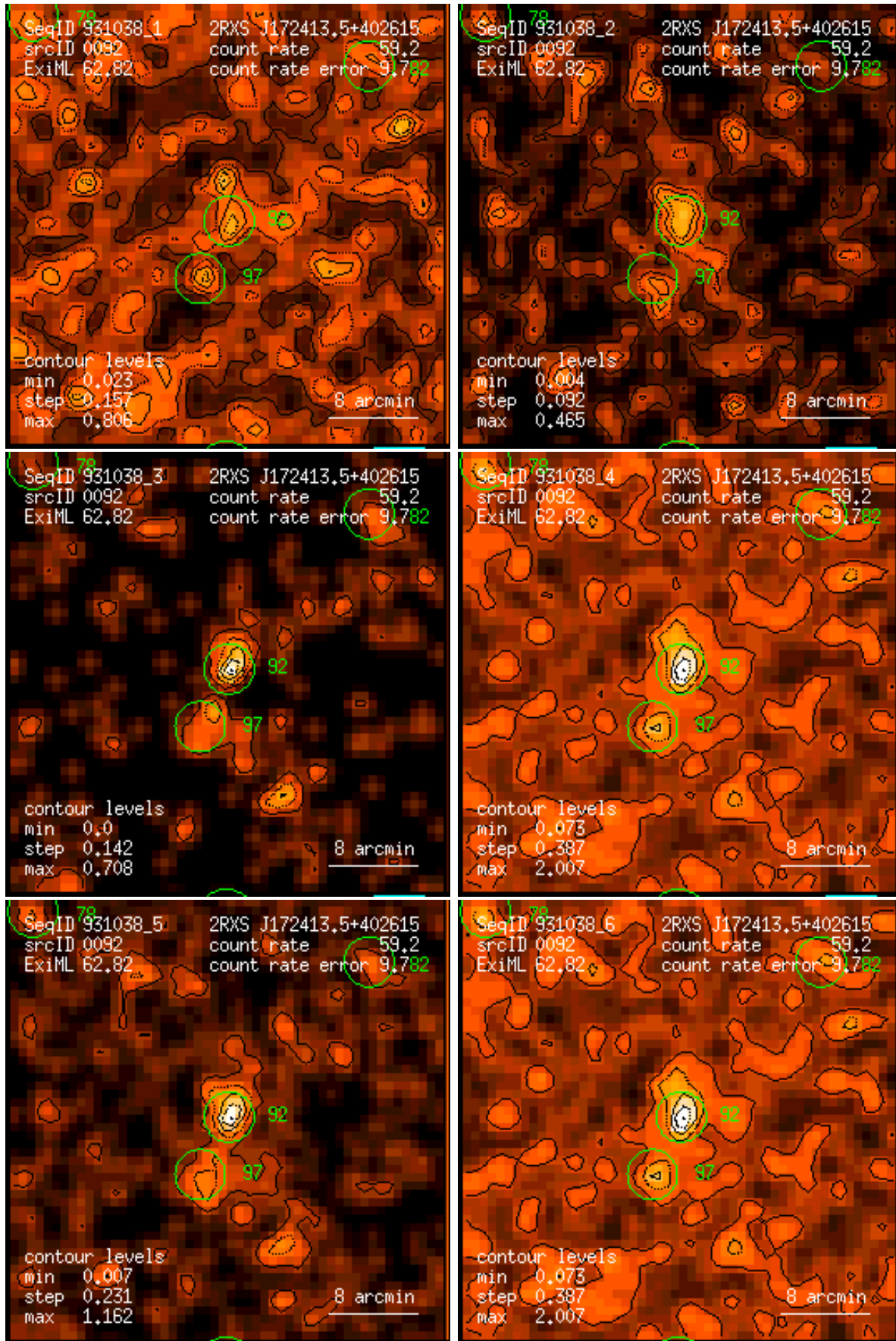
Figure 92: RASS 931038: detection 0092: band rate images, Gaussian filter: (1) PSPC channels 11 – 41, (2) 52 – 90, (3) 91 – 201, (4) 11 – 235, (5) 52 – 201, (6) 11 – 201. Broad band rates in counts/ks. Band rate contour levels in counts/ks/arcmin 2 .
