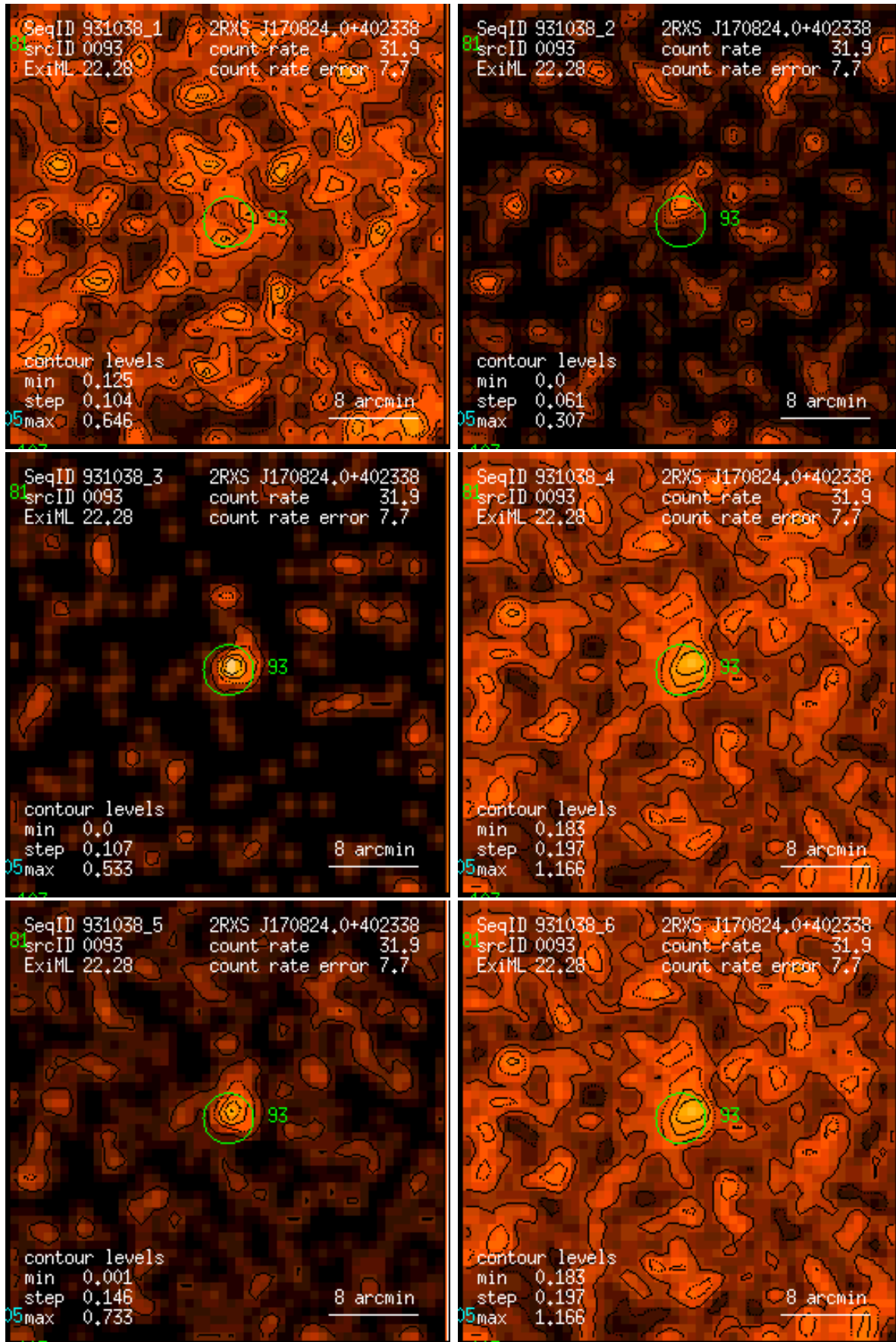
Figure 93: RASS 931038: detection 0093: band rate images, Gaussian filter: (1) PSPC channels 11 – 41, (2) 52 – 90, (3) 91 – 201, (4) 11 – 235, (5) 52 – 201, (6) 11 – 201. Broad band rates in counts/ks. Band rate contour levels in counts/ks/arcmin 2 .
