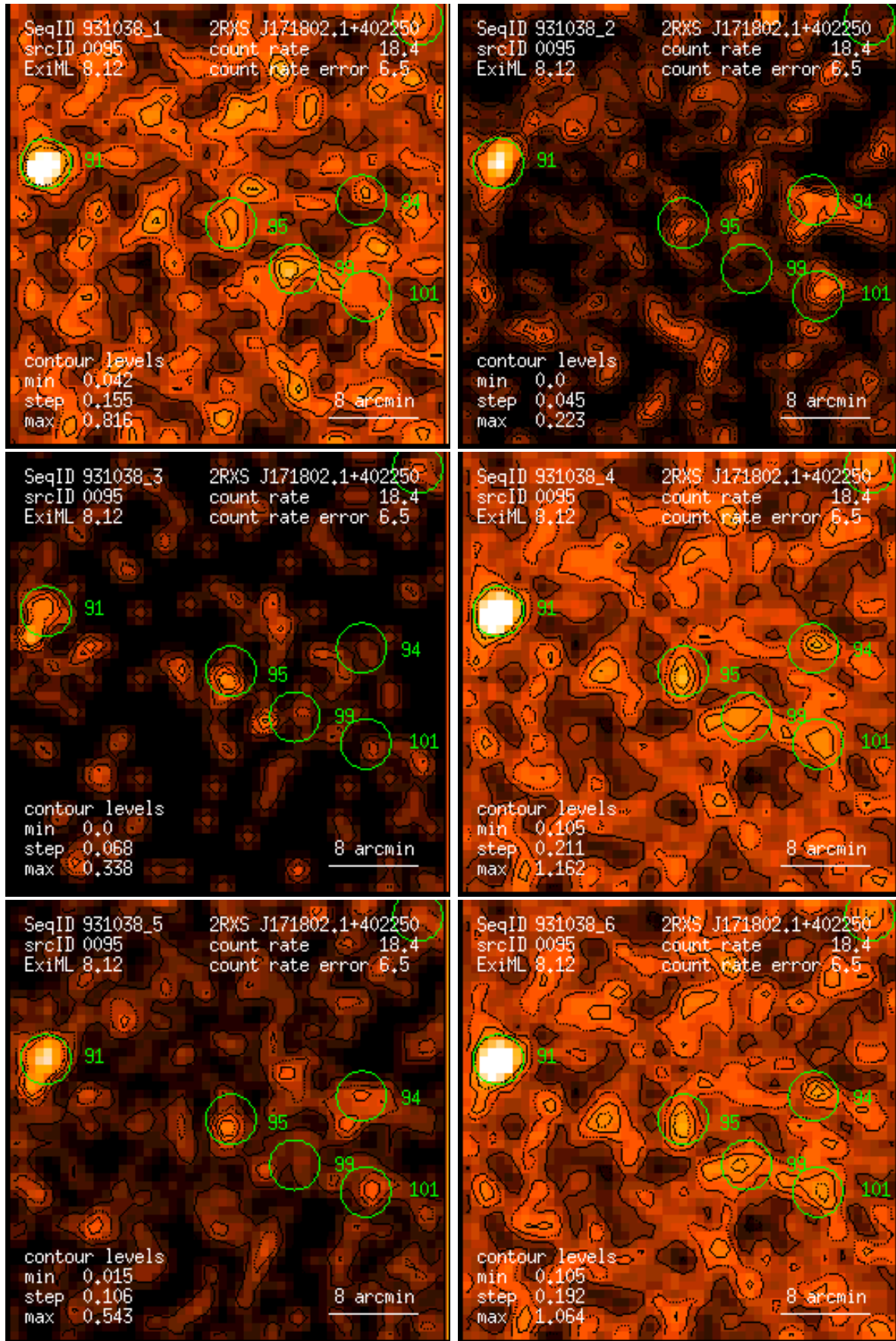
Figure 95: RASS 931038: detection 0095: band rate images, Gaussian filter: (1) PSPC channels 11 – 41, (2) 52 – 90, (3) 91 – 201, (4) 11 – 235, (5) 52 – 201, (6) 11 – 201. Broad band rates in counts/ks. Band rate contour levels in counts/ks/arcmin 2 .
