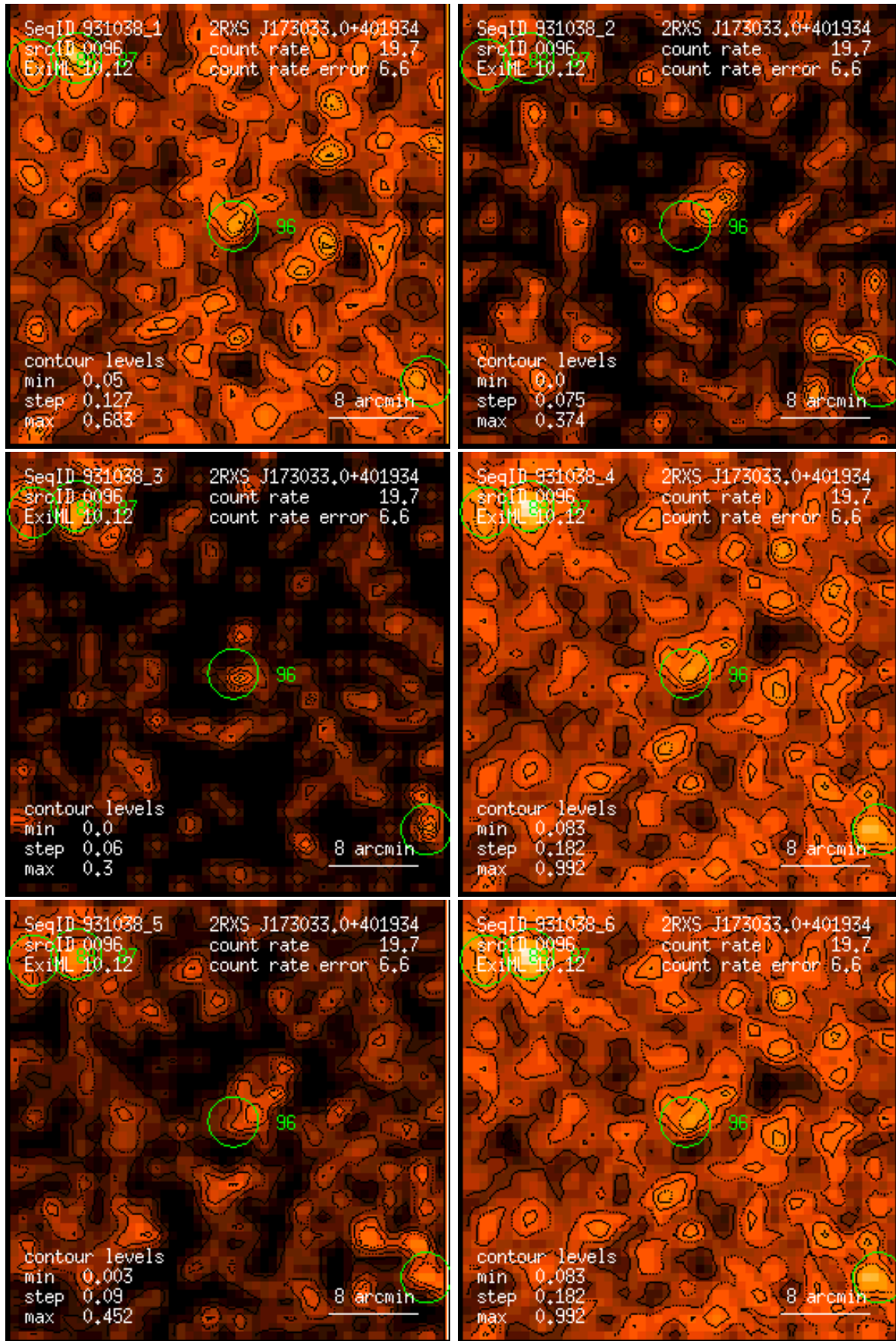
Figure 96: RASS 931038: detection 0096: band rate images, Gaussian filter: (1) PSPC channels 11 – 41, (2) 52 – 90, (3) 91 – 201, (4) 11 – 235, (5) 52 – 201, (6) 11 – 201. Broad band rates in counts/ks. Band rate contour levels in counts/ks/arcmin 2 .
