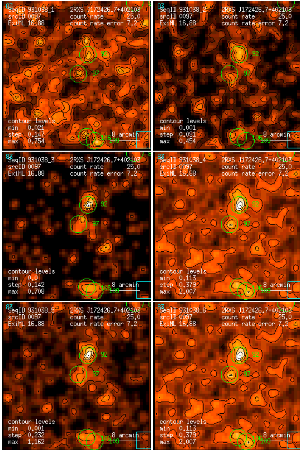
Figure 97: RASS 931038: detection 0097: band rate images, Gaussian filter: (1) PSPC channels 11 – 41, (2) 52 – 90, (3) 91 – 201, (4) 11 – 235, (5) 52 – 201, (6) 11 – 201. Broad band rates in counts/ks. Band rate contour levels in counts/ks/arcmin 2 .
