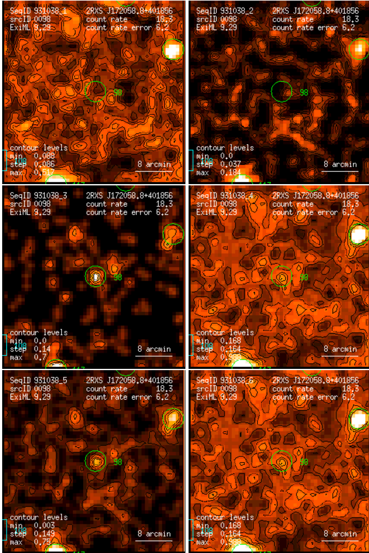
Figure 98: RASS 931038: detection 0098: band rate images, Gaussian filter: (1) PSPC channels 11 – 41, (2) 52 – 90, (3) 91 – 201, (4) 11 – 235, (5) 52 – 201, (6) 11 – 201. Broad band rates in counts/ks. Band rate contour levels in counts/ks/arcmin 2 .
