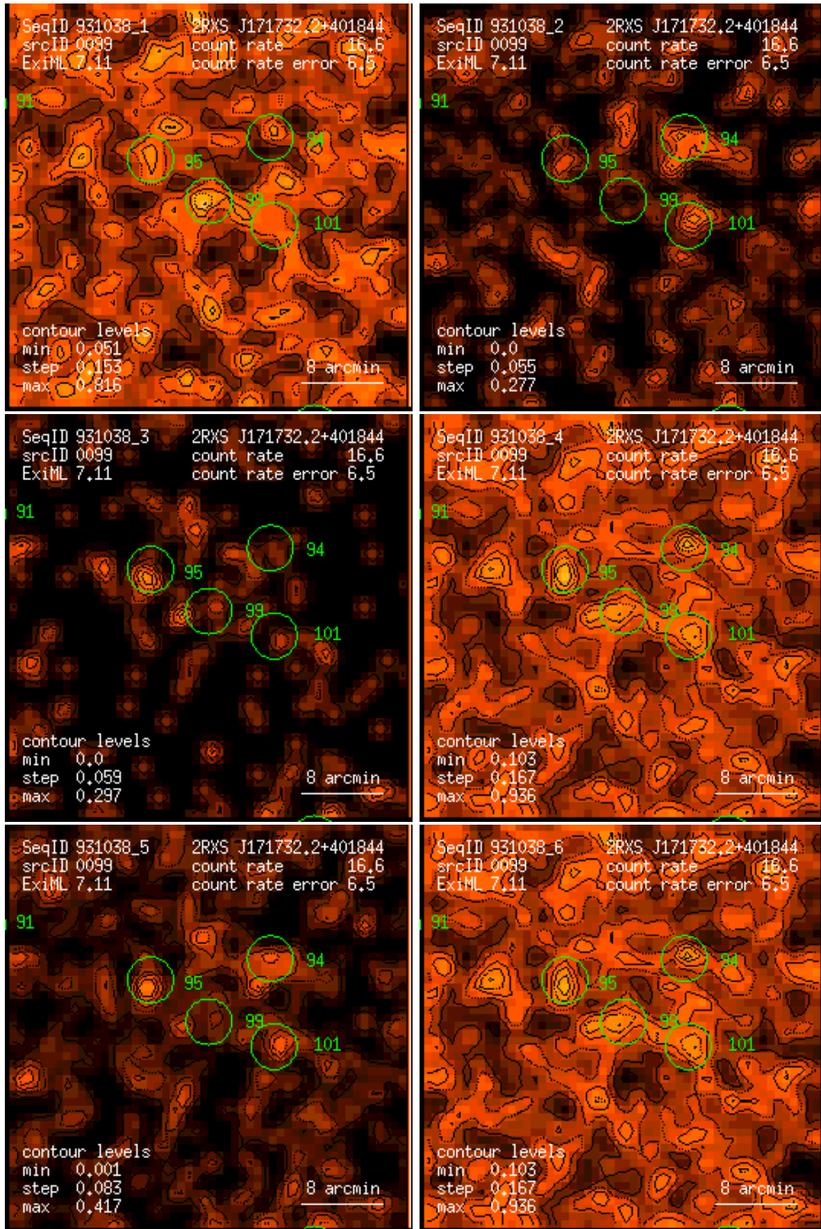
Figure 99: RASS 931038: detection 0099: band rate images, Gaussian filter: (1) PSPC channels 11 – 41, (2) 52 – 90, (3) 91 – 201, (4) 11 – 235, (5) 52 – 201, (6) 11 – 201. Broad band rates in counts/ks. Band rate contour levels in counts/ks/arcmin 2 .
