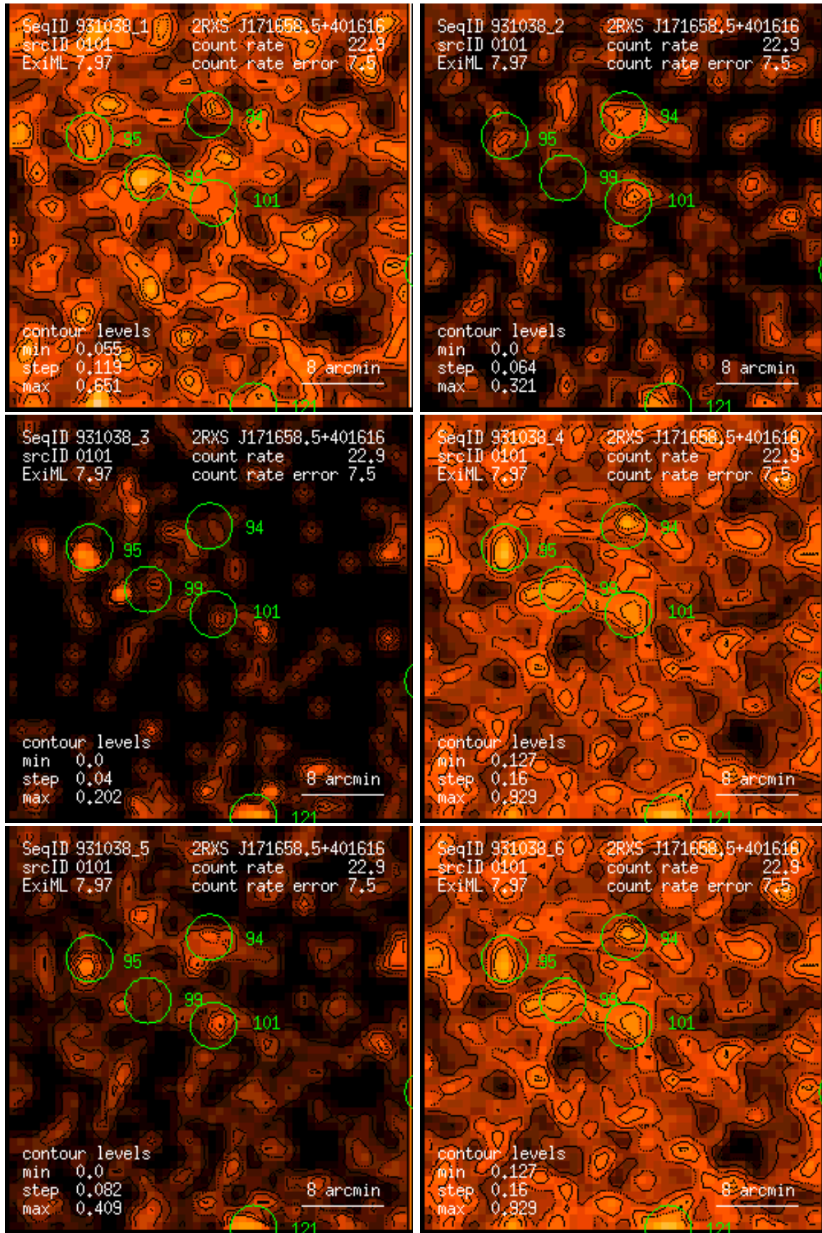
Figure 101: RASS 931038: detection 0101: band rate images, Gaussian filter: (1) PSPC channels 11 – 41, (2) 52 – 90, (3) 91 – 201, (4) 11 – 235, (5) 52 – 201, (6) 11 – 201. Broad band rates in counts/ks. Band rate contour levels in counts/ks/arcmin 2 .
