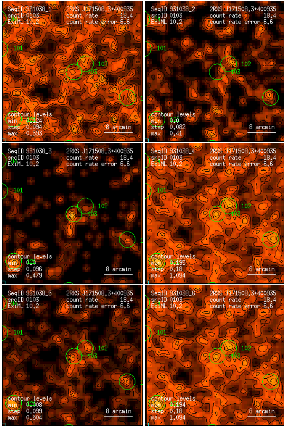
Figure 103: RASS 931038: detection 0103: band rate images, Gaussian filter: (1) PSPC channels 11 – 41, (2) 52 – 90, (3) 91 – 201, (4) 11 – 235, (5) 52 – 201, (6) 11 – 201. Broad band rates in counts/ks. Band rate contour levels in counts/ks/arcmin 2 .
