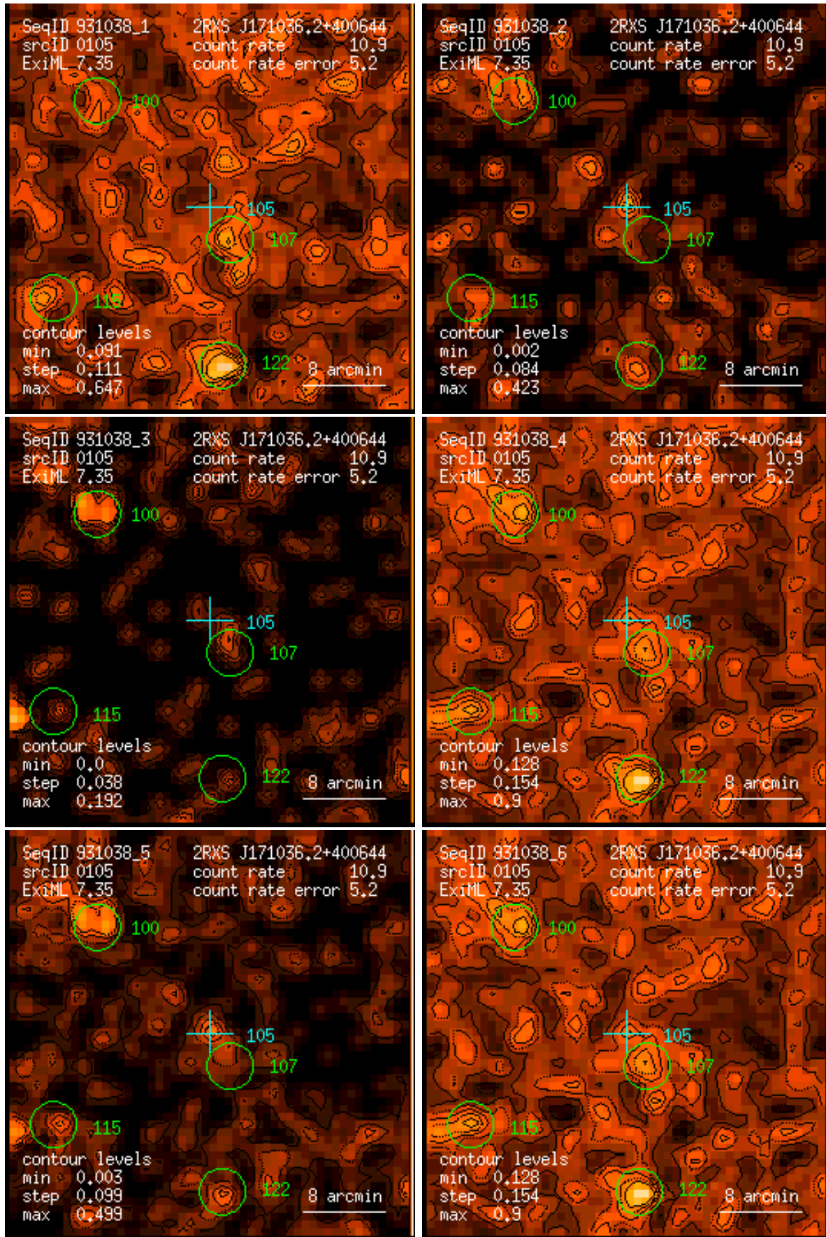
Figure 105: RASS 931038: detection 0105: band rate images, Gaussian filter: (1) PSPC channels 11 – 41, (2) 52 – 90, (3) 91 – 201, (4) 11 – 235, (5) 52 – 201, (6) 11 – 201. Broad band rates in counts/ks. Band rate contour levels in counts/ks/arcmin 2 .
