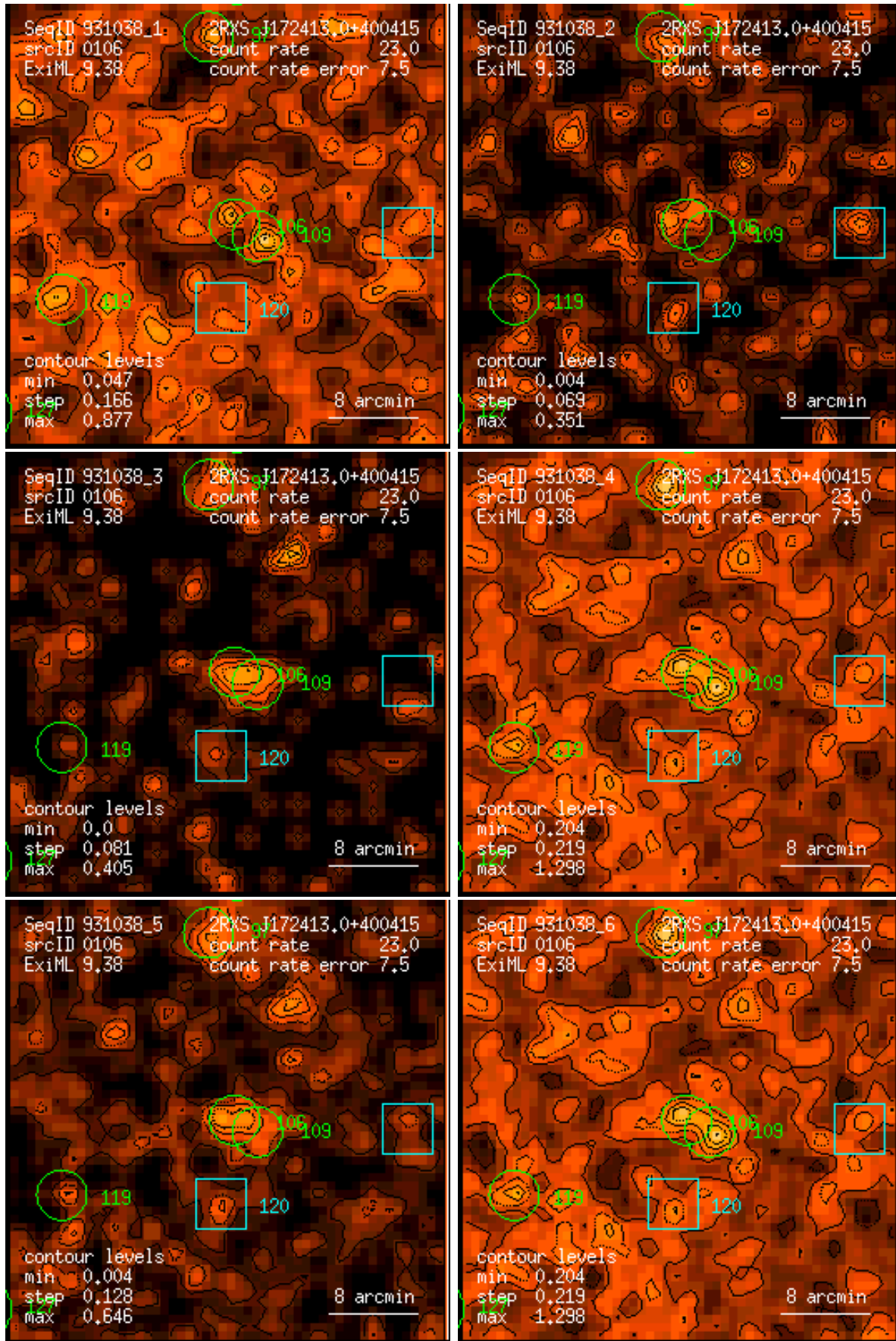
Figure 106: RASS 931038: detection 0106: band rate images, Gaussian filter: (1) PSPC channels 11 – 41, (2) 52 – 90, (3) 91 – 201, (4) 11 – 235, (5) 52 – 201, (6) 11 – 201. Broad band rates in counts/ks. Band rate contour levels in counts/ks/arcmin 2 .
