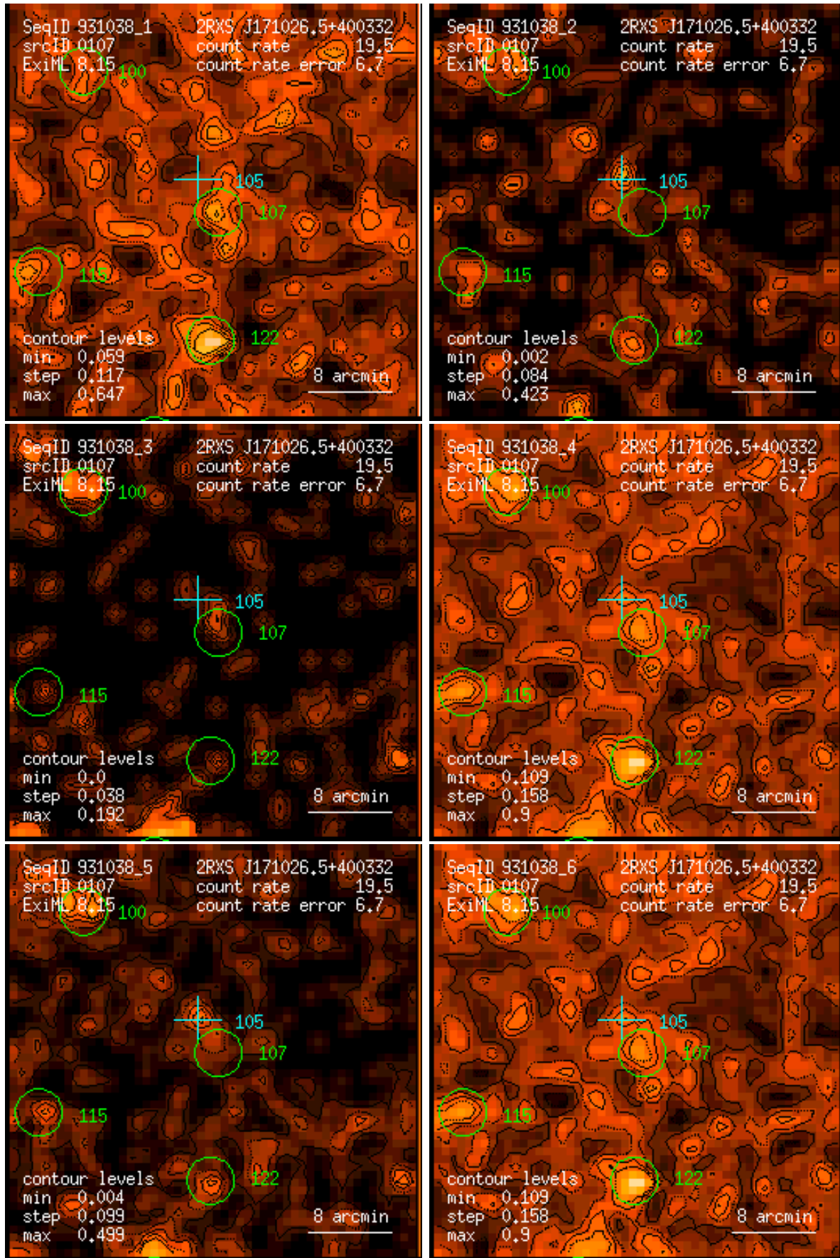
Figure 107: RASS 931038: detection 0107: band rate images, Gaussian filter: (1) PSPC channels 11 – 41, (2) 52 – 90, (3) 91 – 201, (4) 11 – 235, (5) 52 – 201, (6) 11 – 201. Broad band rates in counts/ks. Band rate contour levels in counts/ks/arcmin 2 .
