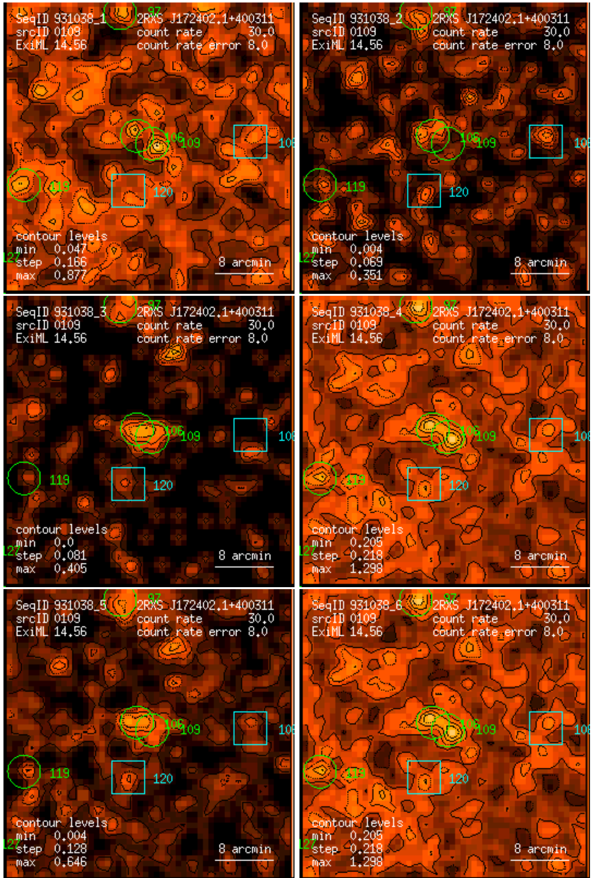
Figure 109: RASS 931038: detection 0109: band rate images, Gaussian filter: (1) PSPC channels 11 – 41, (2) 52 – 90, (3) 91 – 201, (4) 11 – 235, (5) 52 – 201, (6) 11 – 201. Broad band rates in counts/ks. Band rate contour levels in counts/ks/arcmin 2 .
