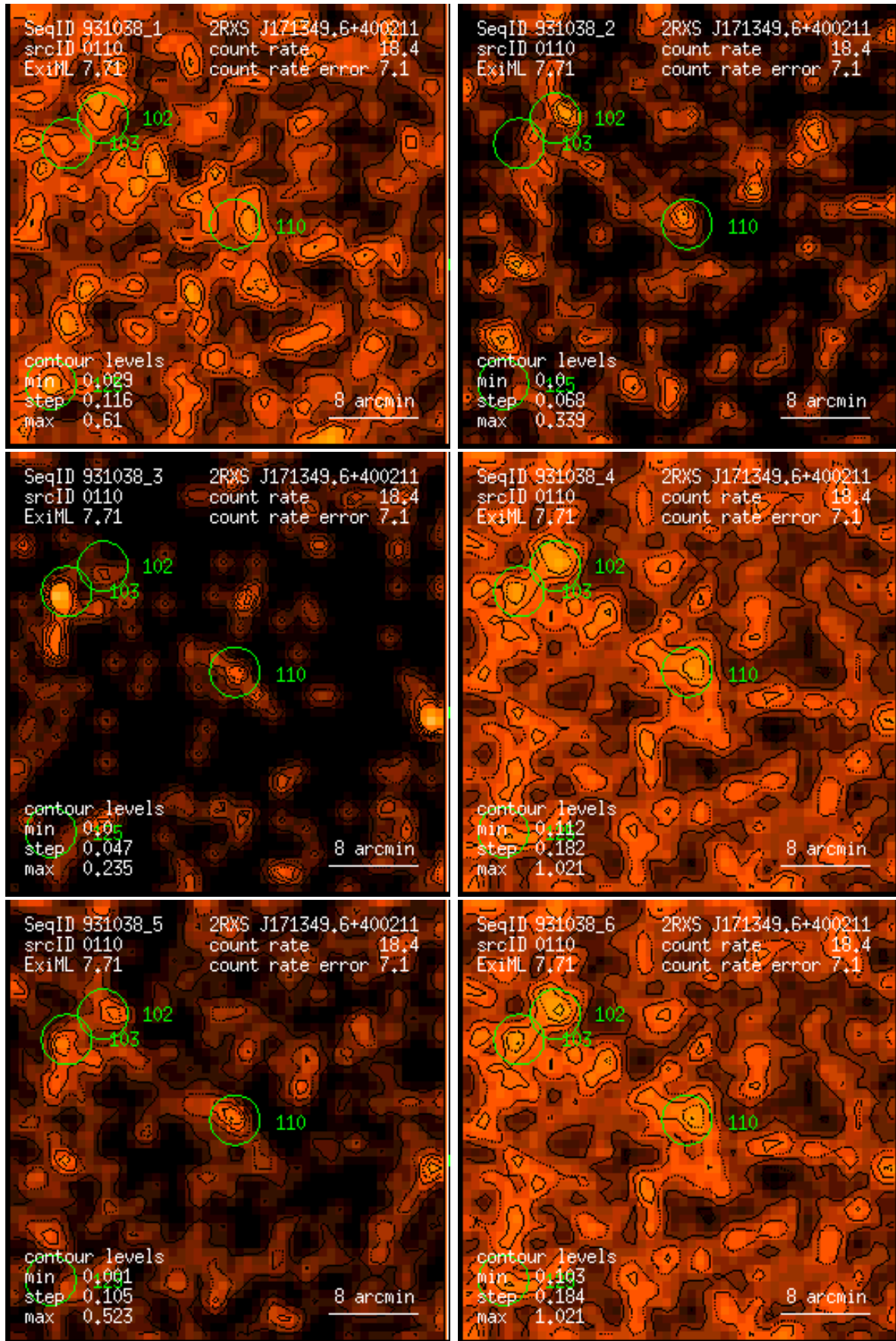
Figure 110: RASS 931038: detection 0110: band rate images, Gaussian filter: (1) PSPC channels 11 – 41, (2) 52 – 90, (3) 91 – 201, (4) 11 – 235, (5) 52 – 201, (6) 11 – 201. Broad band rates in counts/ks. Band rate contour levels in counts/ks/arcmin 2 .
