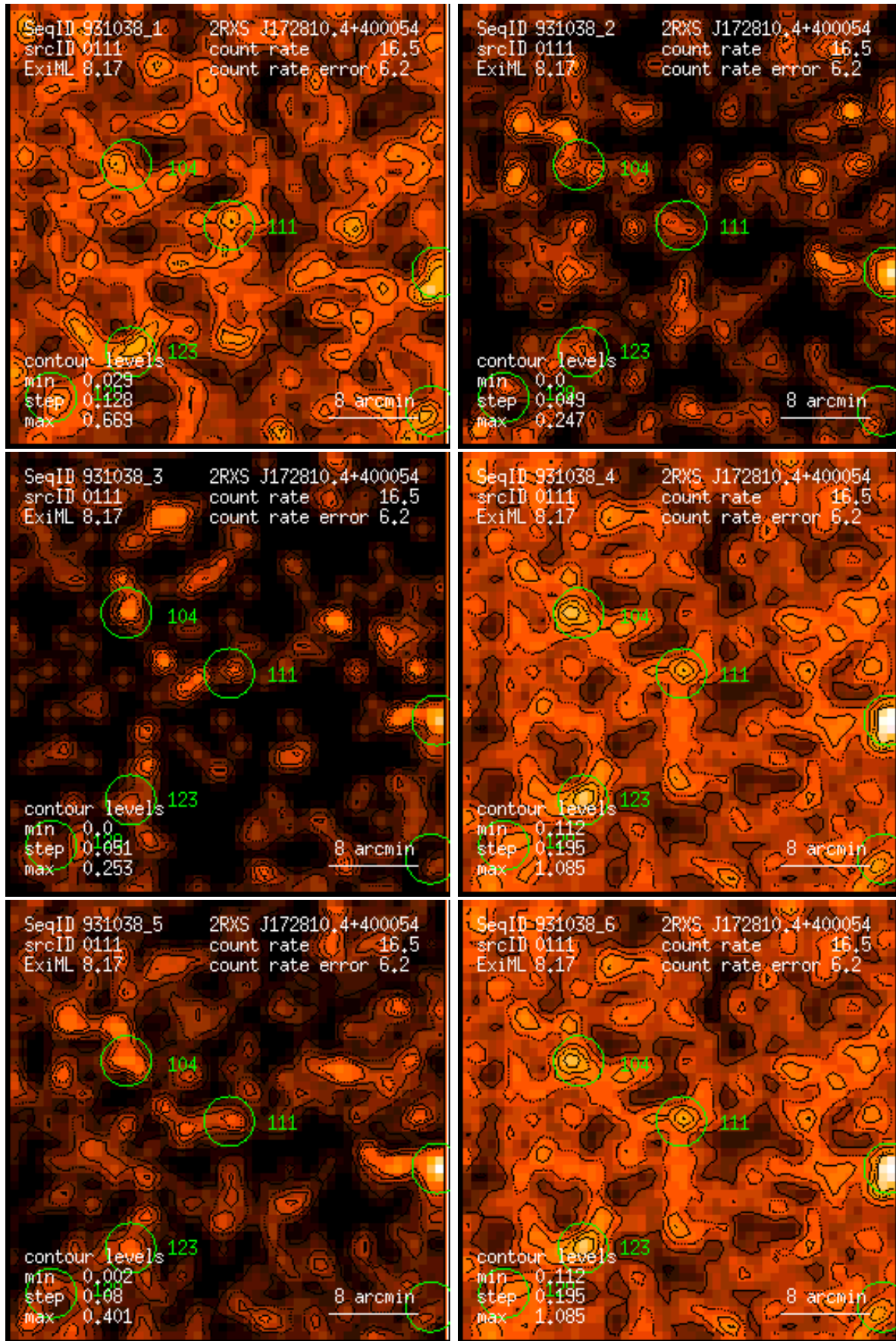
Figure 111: RASS 931038: detection 0111: band rate images, Gaussian filter: (1) PSPC channels 11 – 41, (2) 52 – 90, (3) 91 – 201, (4) 11 – 235, (5) 52 – 201, (6) 11 – 201. Broad band rates in counts/ks. Band rate contour levels in counts/ks/arcmin 2 .
