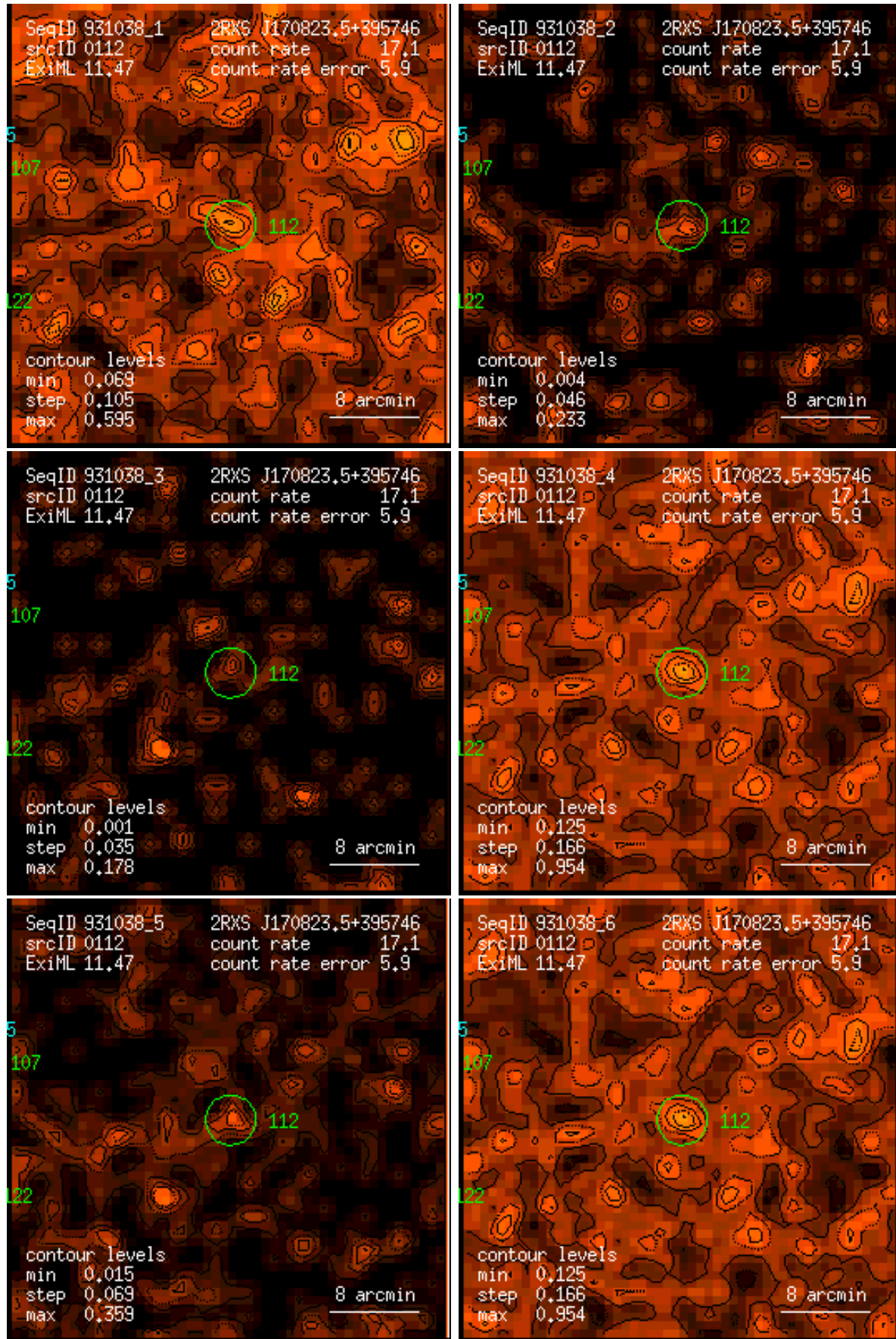
Figure 112: RASS 931038: detection 0112: band rate images, Gaussian filter: (1) PSPC channels 11 – 41, (2) 52 – 90, (3) 91 – 201, (4) 11 – 235, (5) 52 – 201, (6) 11 – 201. Broad band rates in counts/ks. Band rate contour levels in counts/ks/arcmin 2 .
