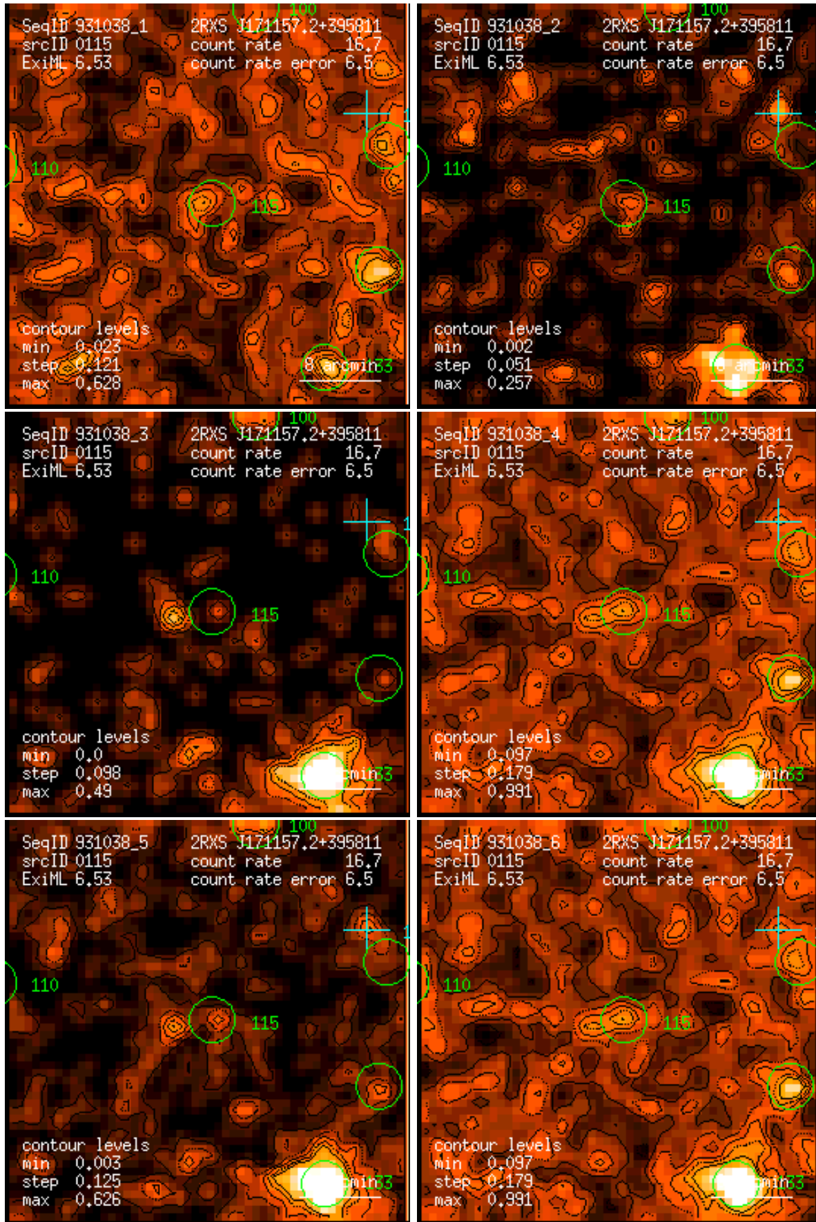
Figure 115: RASS 931038: detection 0115: band rate images, Gaussian filter: (1) PSPC channels 11 – 41, (2) 52 – 90, (3) 91 – 201, (4) 11 – 235, (5) 52 – 201, (6) 11 – 201. Broad band rates in counts/ks. Band rate contour levels in counts/ks/arcmin 2 .
